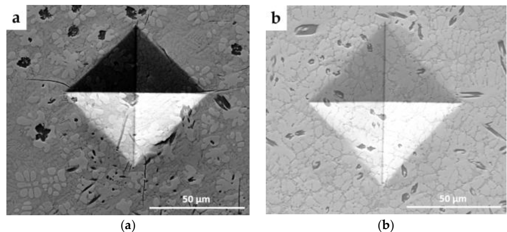
Figure 9. The 2 kgf indentation marks on (a) SL and (b) SH. It can be seen that the deposition of SL demonstrates higher hardness and longer indentation cracks.
