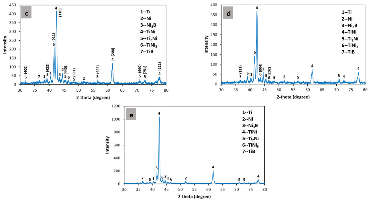
Figure 7. XRD results of (a) Ti-6Al-4V. (b) Deloro-22 powders. (c–e) Sample SL, SM, and SH, respectively.
