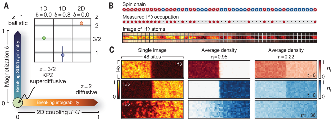
Fig. 1. Hydrodynamic transport in Heisenberg chains and schematic of the experimental system. (A) Dynamical exponents for finite-temperature Heisenberg chains. Whereas integrable systems typically display ballistic transport (magnetized chains, \delta > 0 ), nonintegrable systems are generically diffusive (2D Heisenberg model, J_{\perp} > 0 ). For unmagnetized Heisenberg chains, transport is expected to fall into the KPZ universality class with a superdiffusive exponent z = 3/2 . (Inset) By measuring polarization transfer P(t) across a domain wall, we directly observe these transport regimes: superdiffusion in the unmagnetized case (green), ballistic transport at finite net magnetization (blue), and diffusion in two dimensions (orange). Exponents are extracted by fitting P(t) \propto t^{1/z} ; for the ballistic case, we additionally fit a vertical intercept to account for transient initial-time dynamics. Error bars denote SD of the fit. (B) In each experimental run, we measure the spin states of a Heisenberg
