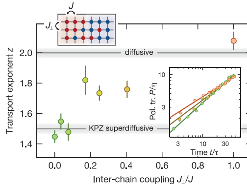
Fig. 3. Evolution toward diffusive transport under a breakdown of integrability. Fitted power-law exponent z for the spin polarization transfer at different coupling strengths between individual 1D chains with initial domain walls with \eta \approx 0.9 (41). Starting from superdiffusive transport in the purely 1D case, z = 1.45(5) , increased interchain coupling breaks the integrability of the system and leads to a crossover toward diffusive transport, reaching z = 2.08(4) in the 2D case, as generically expected for nonintegrable systems. The inset depicts the normalized polarization transfer P(t)/\eta for J_{\perp}/J = 0, 0.40(1) and 1.00(5) (green to orange). Error bars denote SD of the fit.
