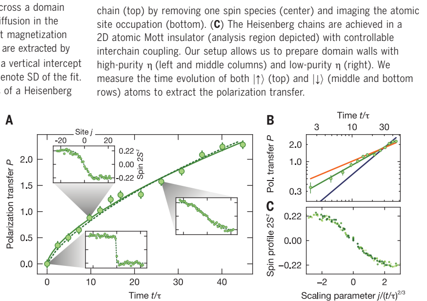
Fig. 2. Superdiffusive spin transport in a high-temperature Heisenberg chain. (A) The polarization transfer for a domain-wall initial state with a contrast of \eta = 0.22(2) grows as a power law [ P(t) \propto t^{1/z} ] with a fitted exponent z = 1.54(7) (solid line), indicating superdiffusive transport. The experimental data are consistent with numerical Heisenberg-model simulations (41) (dashed line). The insets show the averaged spin profiles 2S_j^z(t) at times t/\tau = 0, 10, 26 , which are compared to simulations (dashed lines). (B) Polarization transfer in a double-logarithmic plot. The solid lines are power-law fits with fixed exponents, where a distinction between z = 3/2 (green) and both z = 2 (brown) and z = 1 (blue) is visible. (C) When rescaling time by the inverse dynamical exponent, the spatial spin profiles at times t/\tau = 5 to 35 (light to dark green) collapse to a characteristic shape consistent with the integrated KPZ function. Error bars denote SEM.
