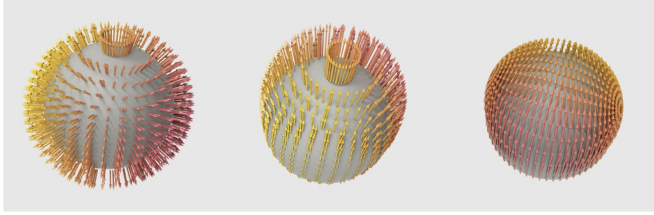
FIG. 9. Minimizers for \kappa negative. • (Left) \kappa = -8 • (Center) \kappa = -4 • (Right) \kappa = -2 .
