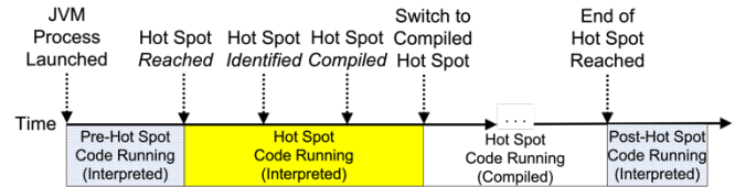
Fig. 12. Execution Timeline of HotSpot-Optimized CircuitSolver.java
