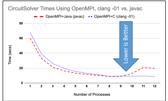
Fig. 11. Runtimes of circuitSolver.c (-O1 Optimized) and CircuitSolver.java
