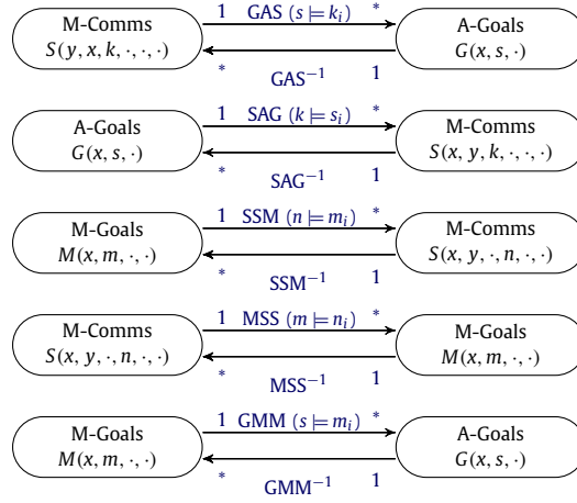
Fig. 8. Functions relating (s-)comms and (m-)goals.
