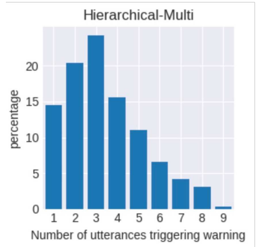
Figure 5: Percentage of the number of utterances elapsed when the model makes a positive prediction of derailment.
