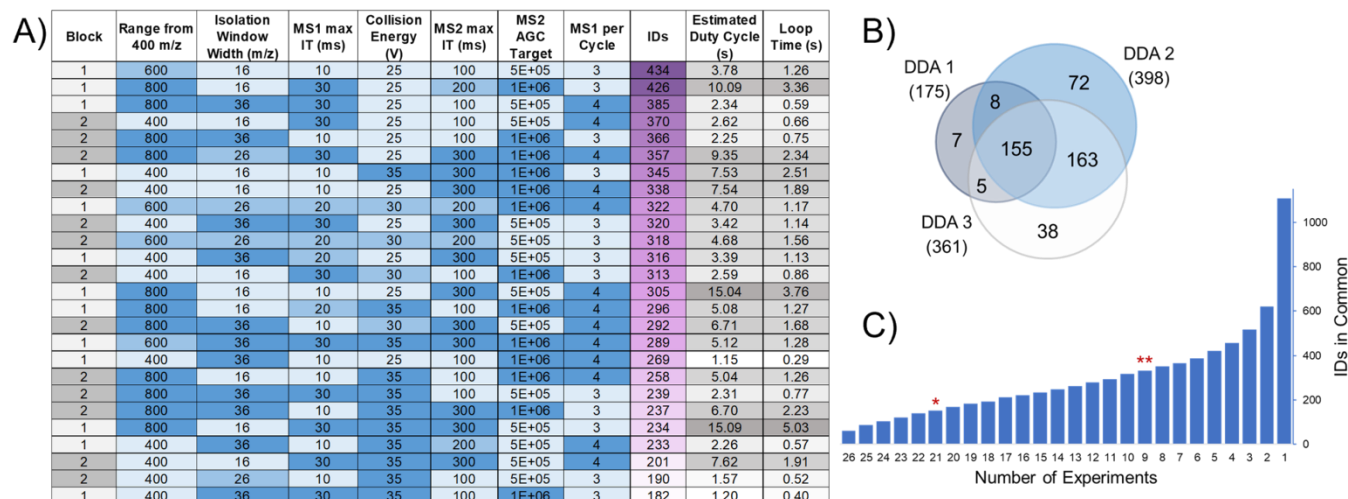
Figure 1. A) Peptide identifications resulting from 26 DIA acquisitions outlined by the DSD. B) Overlapping peptide identifications from triplicate DDA acquisitions are shown. C) Bar chart describing the number of overlapping peptides in different numbers of DIA acquisitions. Red
