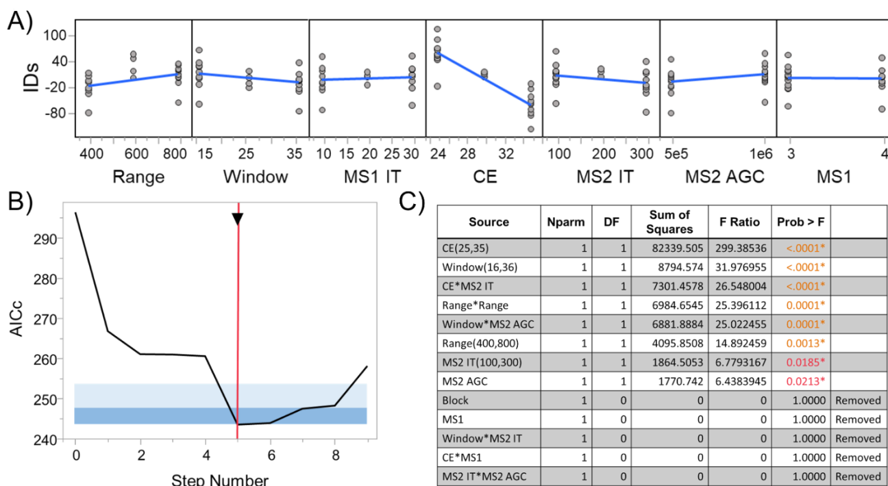
Figure 2. Fit definitive screening to identify parameter effects. A) Main effects residual plots of the tested parameters are shown. B) Solution path for the generalized regression models were evaluated using AICc where C) the minimum AICc value resulted from this table of main and even-order effects.
