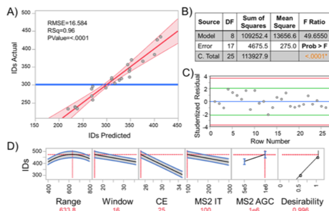
Figure 3. A) Model validation was performed by comparing the predicted IDs to the observed IDs. B) Analysis of variance was calculated to determine the model as significant. C) Externally studentized residuals are shown with 95% simultaneous limits calculated through the Bonferroni method (red lines) and individual limits (green lines). D) Optimal parameter values were predicted through maximizing the desirability of the model, with confidence limits shown.
