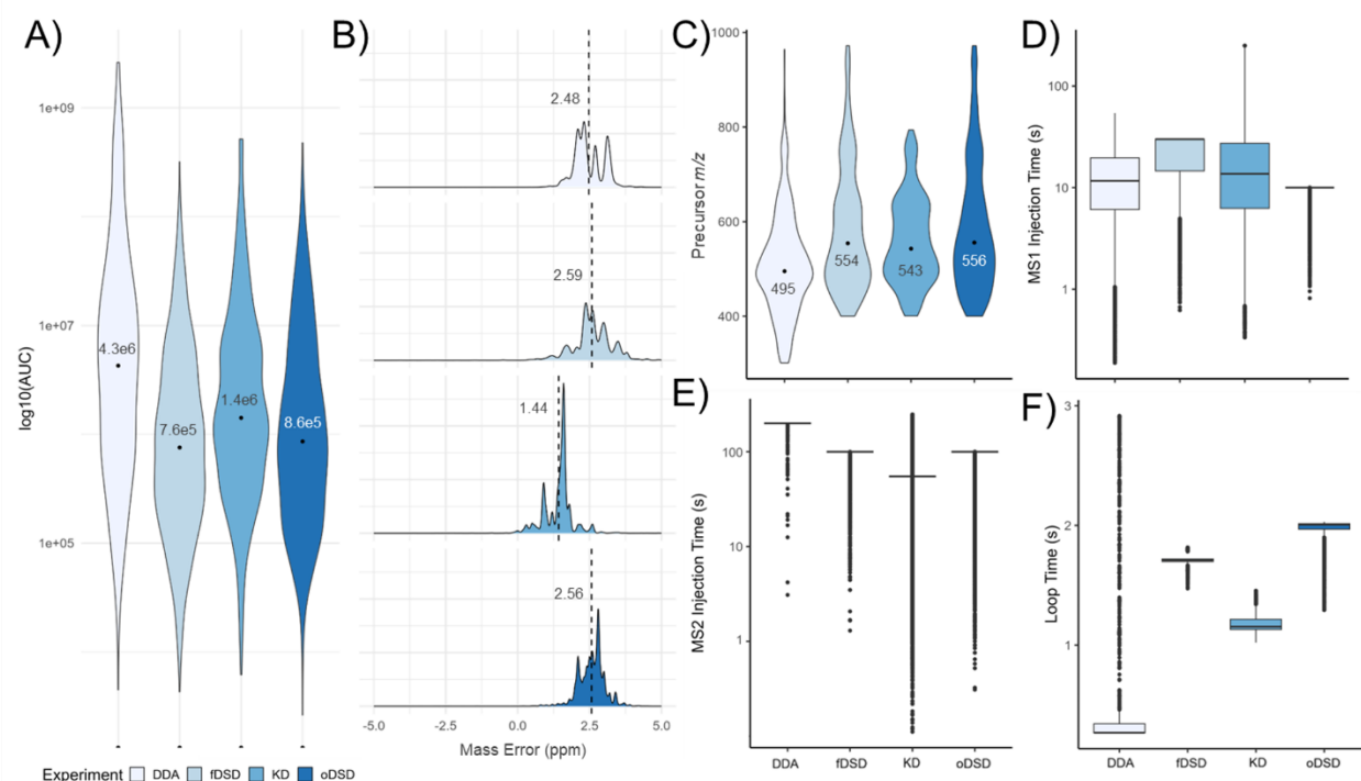
Figure 5. Comparison of figures of merit between methods and detected neuropeptides. A) Log10 transformed neuropeptide AUC distributions. B) Distributions of identification mass error. C) Precursor m/z distributions. D) MS1 and E) MS2 injection times. F) Loop time between MS1 scans.
