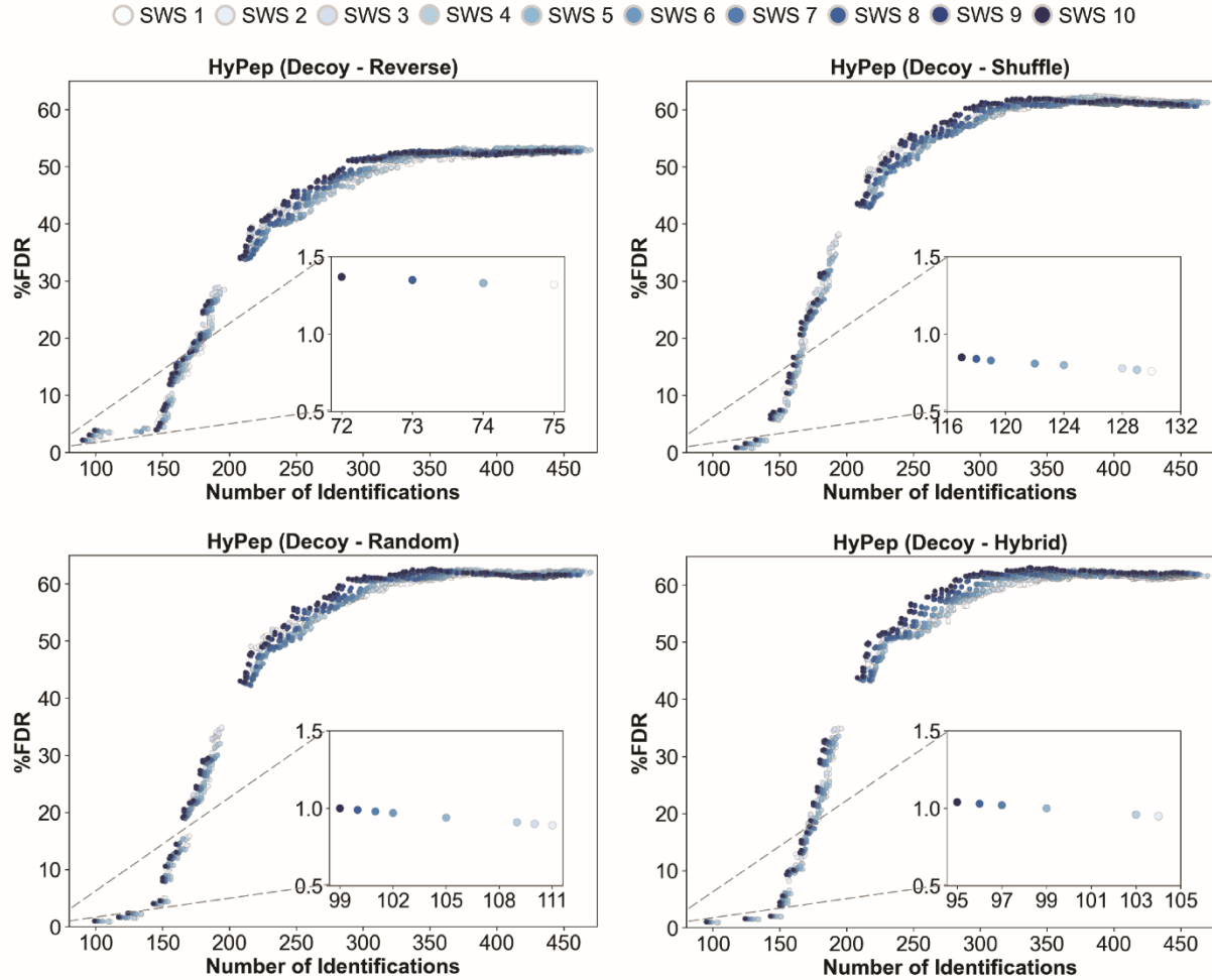
Figure 3. Neuropeptide identifications as a function of % FDR from C. sapidus brain tissue processed using HyPep, which contains four target-decoy methods to calculate % FDR. Decoy databases can be generated using either shuffle, reverse, random, or hybrid decoy methods for FDR calculation ( Figure S1 ). Insets show magnification at 0.5-1.5% FDR. Each color represents different sliding window sizes (SWS). For each target-decoy method, the same decoy database was used for neuropeptide identification using SWS values 1-10.
