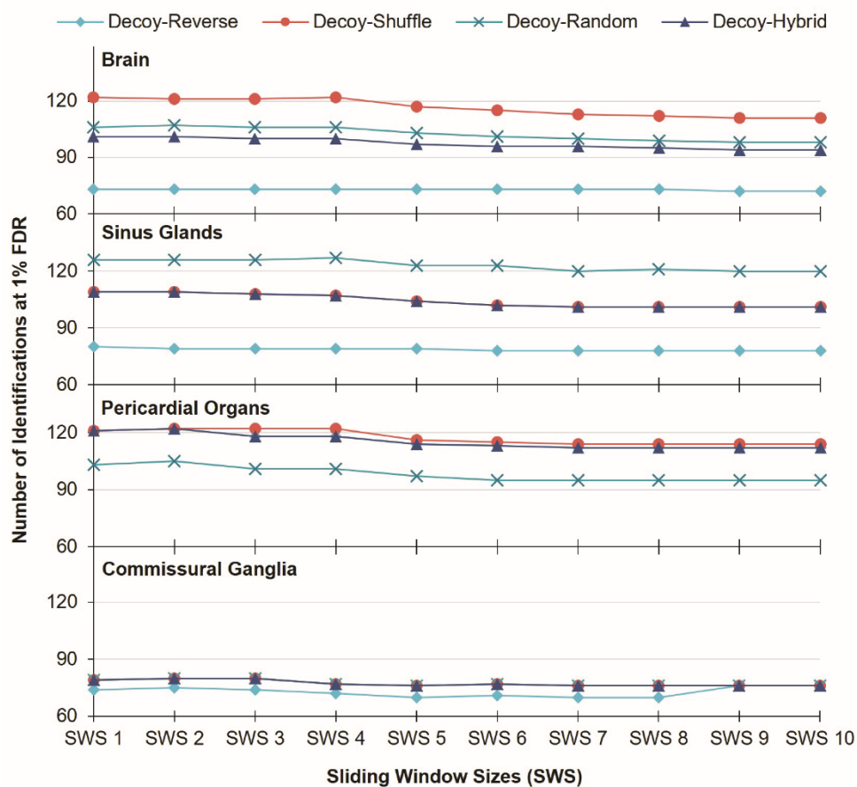
Figure 4. Four tissues from C. sapidus (brain, sinus glands, pericardial organs, and commissural ganglia) were processed using HyPep parameters at SWS values 1-10 and four target-decoy methods (reverse = diamond, circle = shuffle, x = random, and triangle = hybrid). The number of identifications for each tissue using each SWS value and each target-decoy method are reported at threshold of 1% FDR.
