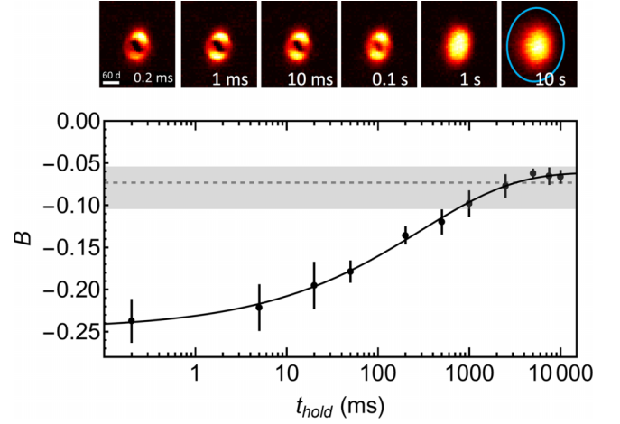
FIG. 2. Relaxation of the density profile. A series of images taken for s = 7E_R is shown, with corresponding measurements of B , for different times after the optical barrier potential is removed. Mardia's B increases towards the equilibrium value over long times as the hole disappears from the density profile. The error bars show the standard deviation for the four to six measurements averaged at each hold time. The gray dashed line shows B for a Gaussian distribution, and the gray bar displays the range of B values expected for a gas in equilibrium (see Appendix C). The elliptical mask used to suppress the effect of imaging noise is superimposed (light blue) for the image at t_{\text{hold}} = 10 s. The solid black line is a fit to a stretched exponential. The stretched exponential fits the data well for all lattice depths with adjusted R^2 values ranging from 0.87 to 0.97.
