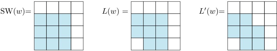
FIGURE 2. \text{SW}(w) , L(w) and L'(w) for w = 3412 .
