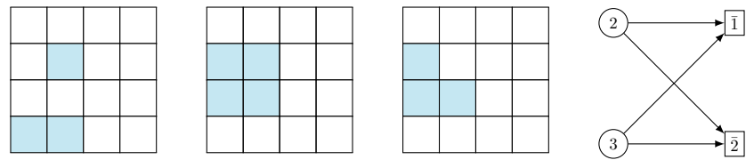
FIGURE 3. D^\circ(w) , L(w) , L'(w) , and G^w for w = 3142 .
