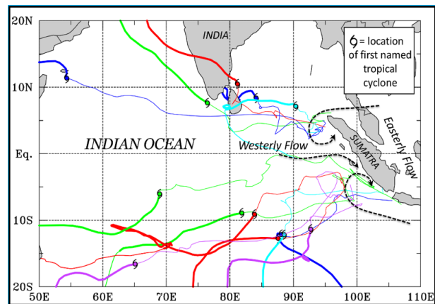
Fig. 6. Tracks of the 13 shed vortices from northern and southern Sumatra that eventually formed named tropical cyclones. TC tracks are based on Joint Typhoon Warning Center (JTWC) best track data and NOAA's International Best Track Archive for Climate Stewardship (IBTrACS). Dashed arrows depict typical low-level flow patterns associated with vortex shedding for the TC cases. One-quarter of the TCs during the DYNAMO/YOTC period originated from shed vortices
