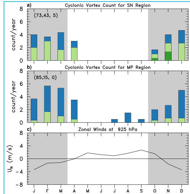
Figs. 3(a-c). Monthly frequency of terrain-induced shed (top of light green bars) and non-shed (length of blue bars) cyclonic vortices for (a) Sumatra north (SN), (b) Malay Peninsula (MP) regions and (c) Monthly mean zonal wind speed ( ms^{-1} ) along 100^\circ E (line segment shown in Fig. 1), indicating most cyclonic vortices in these regions occur in mean easterly flow during the boreal winter monsoon. TC events originating from terrain-induced vortices shown in dark green. Gray shading indicates period with three years of data from both YOTC and DYNAMO; unshaded period has only two years of YOTC data. Numbers in parentheses indicate total wake vortex counts, number of wake vortices that are shed and number that became TCs, respectively. From Fine et al. (2016)
