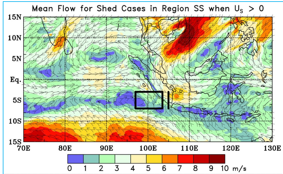
Fig. 7. Mean 925-850 hPa flow over Indian Ocean basin for shed vortices from region SS (black box shown) under conditions of westerly (7 cases) flow in the analysis region. U_s is the mean zonal flow along the vertical black line segment at 105° E
