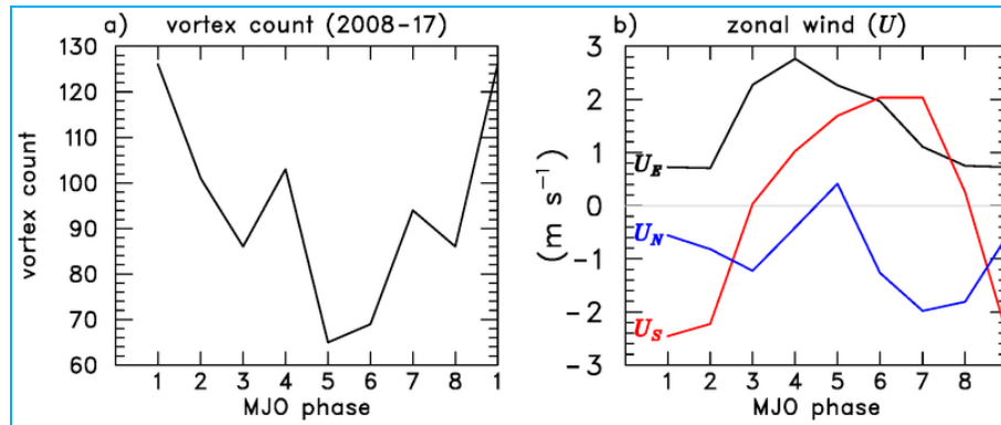
Figs. 8(a&b). Statistics for the period 2008-17 as a function of MJO phase: (a) vortex count for four regions depicted in Fig. 2 and (b) 925-hPa zonal winds along red line segments shown in Fig. 1. Black curve represents zonal winds averaged across the equator ( U_E ), blue curve over northern Sumatra ( U_N ) and red curve over southern Sumatra ( U_S )
