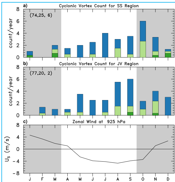
Figs. 4(a-c). As in Fig. 3, except for (a) Sumatra south (SS) and (b) west Java (JV) regions. (c) Monthly mean zonal wind ( \text{m s}^{-1} ) along 105° E (line segment shown in Fig. 1), indicating cyclonic vortices in these regions can occur during both easterly and westerly mean flow. From Fine et al. (2016)
