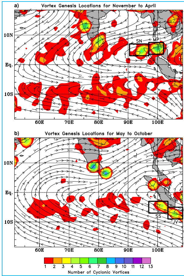
Figs. 2(a&b). Frequency of cyclonic vortex genesis on a 1^\circ grid for (a) November-April and (b) May-October periods for YOTC/DYNAMO period. Streamlines depict 925-850 hPa layer-average flows. Flows in (a) and (b) typify boreal winter and summer monsoon conditions, respectively. From Fine et al. (2016)
