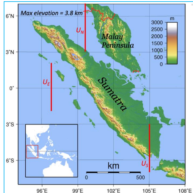
Fig. 1. Topography of Sumatra and surrounding region. Red line segments labeled U_N , U_E and U_S denote the regions over which the zonal flow U is averaged upstream of northern Sumatra (N), west of Sumatra along the equator (E) and at the southern end of Sumatra (S), respectively
