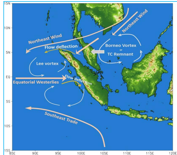
Fig. 9. Synoptic conditions favorable for the formation of lee vortices to the west of Sumatra that may subsequently develop into TCs in the IO during October-December. These factors include vorticity and moisture advection from the South China Sea linked to TC remnants or Borneo vortices, prevailing northeasterly (southeasterly) winds in NH (SH) and the deflection of low-level northeasterly wind by the northern part (westerly wind by the southern part) of Sumatra for the northern (southern) vortex. From Wang et al. (2020)
