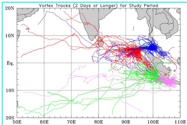
Fig. 5. Tracks for cyclonic vortices that survived more than two days originating from the four analysis regions during YOTC/DYNAMO period: Sumatra north (SN, red), Malay Peninsula (MP, blue), Sumatra south (SS, green) and west Java (JV, purple). From Fine et al. (2016)
