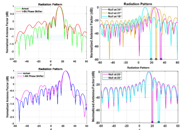
Fig 3. Comparison of a 1-bit phase shifter beamformer with a 6-bit beamformer's beam steering and nulling performance of a 20 \times 20 array.
