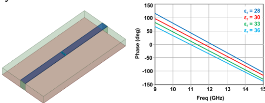
Fig. 5. BST - based microstrip phase shifter: (a) schematic of the design, (b) simulated phase shifts in degrees for different values of dielectric constant.
