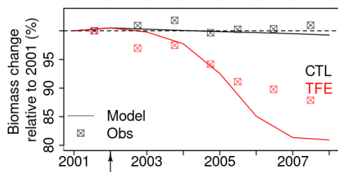
Figure 9. Tree biomass change simulated by model after mortality being triggered. The squares in the plot denote the observation. Biomass change relative to 2001 is calculated by dividing biomass during 2002–2008 by biomass in 2001.
