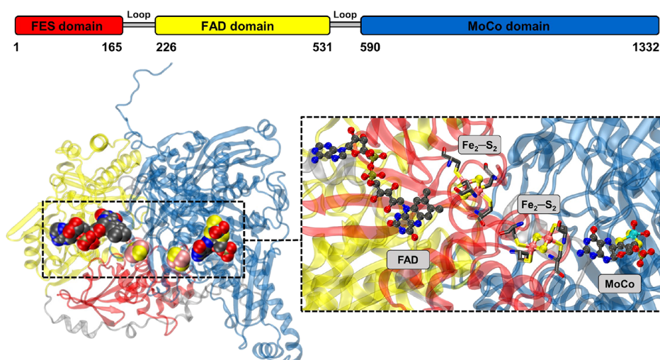
Figure 1. One subunit of the bovine xanthine oxidoreductase homodimer (PDB ID: 1JRO). 47 The close-up represents the XOR's active regions in the redox reaction that are almost linearly positioned in the order of MoCo, Fe 2 -S 2 , and FAD. Hydrogen atoms are not presented for more clarity, and four cysteine residues bound to the Fe 2 -S 2 cluster's irons are shown in the sticks.
