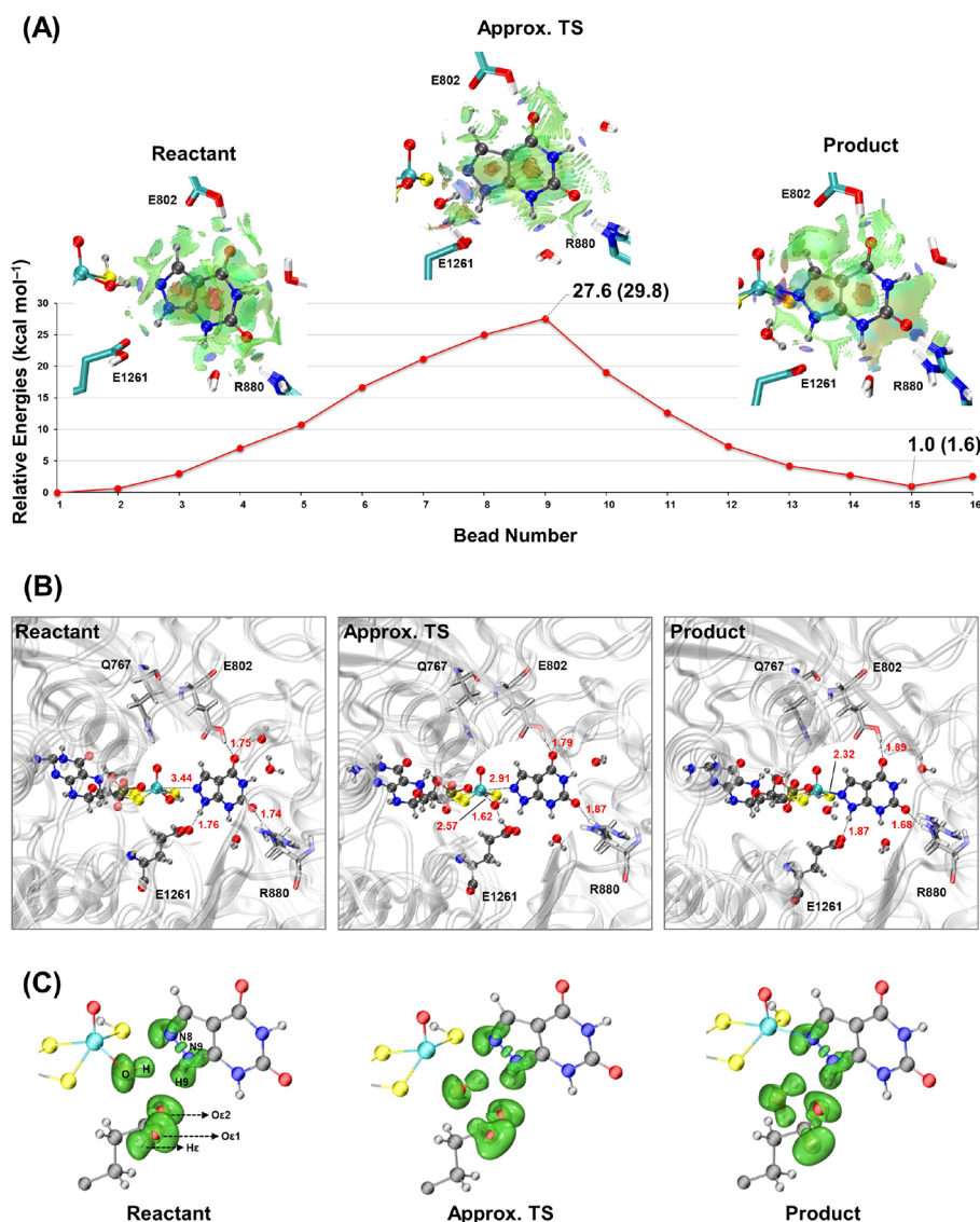
Figure 4. (A) Minimum energy path for the catalytic inhibition of XO by oxipurinol modeled via the QSM together with the NCI plots of the critical structures. The QM/MM optimization energies (kcal mol -1 ) are calculated at the \omega B97X-D/def2-SVP level of theory with the AMBER ff14SB force field. The values in parenthesis correspond to the Gibbs free energies obtained from the vibrational analysis using Eyringpy. (B) Optimized geometries of the critical structures with the values of selected distances (Å). (C) ELF basins among the MoCo, oxipurinol, and E1261 for the critical structures along the reaction pathway.
