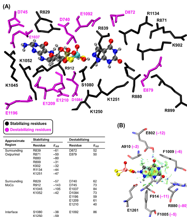
Figure 3. (A) Residues of the XO-OXI active site with considerable non-bonded intermolecular interactions ( |E_{NB}| \geq 30 kcal mol -1 ). Residues in the sticks have stabilizing (black) and destabilizing (purple) interactions with the active site, given in the ball-and-sticks. E1261 of the active site is not shown for enhanced clarity. (B) Plot of the aNCI between the inhibitor and the surrounding residues of the active site. Values in parenthesis correspond to E_{NB} (kcal mol -1 ) of each residue.
