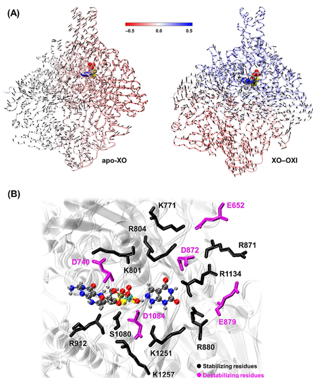
Figure 2. (A) Plots of the PCA on the root-mean-square fluctuations (first mode) along with the residue-wise correlation with respect to MoCo as a heatmap projected on the protein for the apo-XO and XO-OXI. The black arrows show the fluctuations greater than 1.0 Å and point toward the direction of the highest ranked eigenvector, and their amplitude is directly proportional to the length of the arrow. Areas with correlated movements in the heatmap are colored blue (0.5), non-correlated areas are white (0.0), and anti-correlated movements are red (−0.5). (B) Representation of the residues with considerable non-bonded intermolecular interactions ( |\Delta E_{NB}| \geq 12.0 kcal mol -1 ) with the MoCo of XO-OXI compared to that of the apo-XO as the reference.
