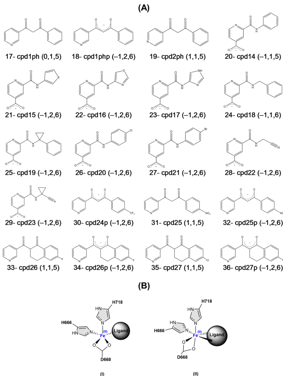
Scheme 2. (A) Second Set of the Studied Ligands a and (B) Different Geometries of the Active Site in Coordination with the Lead Compounds
