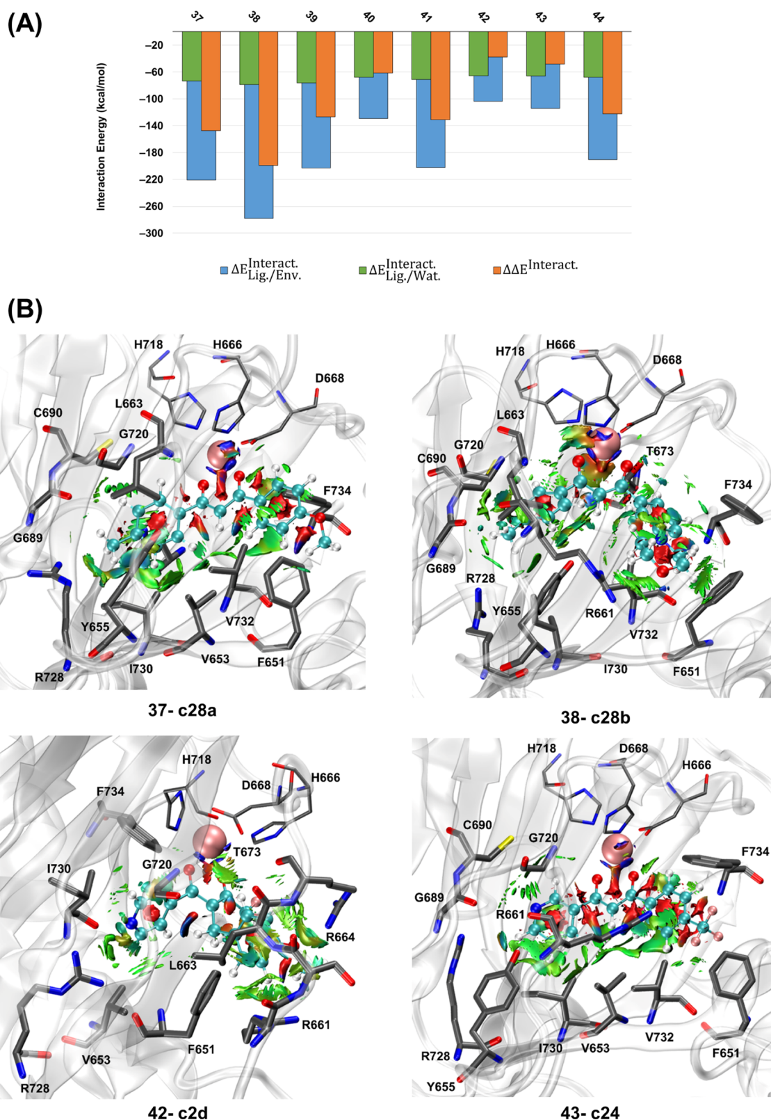
Figure 6. (A) Calculated QM/MM interaction energies ( \text{kcal mol}^{-1} ) for the most stable representative of the studied ligands of the third set (ID: 37–44) at the \omega B97X-D/6-31G(d,p) level of theory and AMOEBAbio18 force field. (B) Averaged noncovalent interactions (aNCIs) between the ligand and its surrounding residues for c28a, c28b, c2d, and c24. The isosurface cutoff for the NCI is 0.35 au, and the data is plotted in the color range of -0.05 < \text{sign}(\lambda_2)\rho < 0.05 au. Residues H666, D668, and H718 are shown in thin sticks, ligand atoms are in ball and sticks (with different color codes), \text{Fe}^{2+} is in pink vdW sphere, and the surrounding residues with the noncovalent interactions are in thick sticks. Hydrogen atoms are not shown for more clarity.
