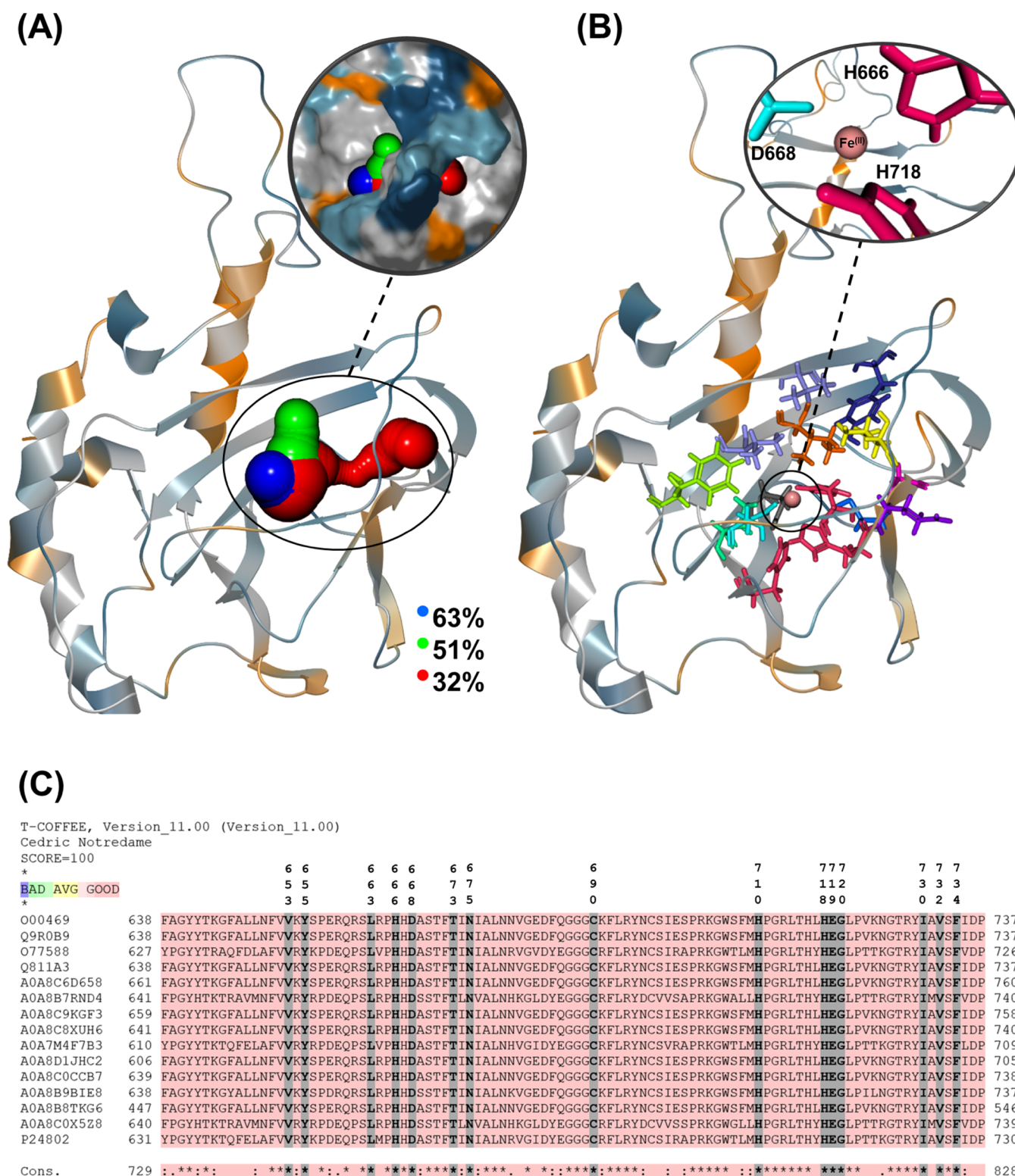
Figure 4. (A) O 2 -transporting tunnels with the largest calculated percentages along the trajectory observed in the apoenzyme. Calculated tunnels are colored in blue, green, and red based on the tunnel's length (blue: shortest, red: longest). The intersection of the tunnels inside the protein is the active site, which is not shown for clarity. The molecular surface of the protein is shown in magnification to give a better view of the enzyme's cavities. (B) Close-up of the approximate positions of the tunnel-lining residues with more than ~80% presence in all of the calculated tunnels/representatives. (C) Condensed sequence alignment between human LH2 (UniProtKB: O00469) and selected members of the LH family. Key: “*” indicates residues conserved in all of the sequences, while “:” and “.” indicate highly and weakly conserved residues.
