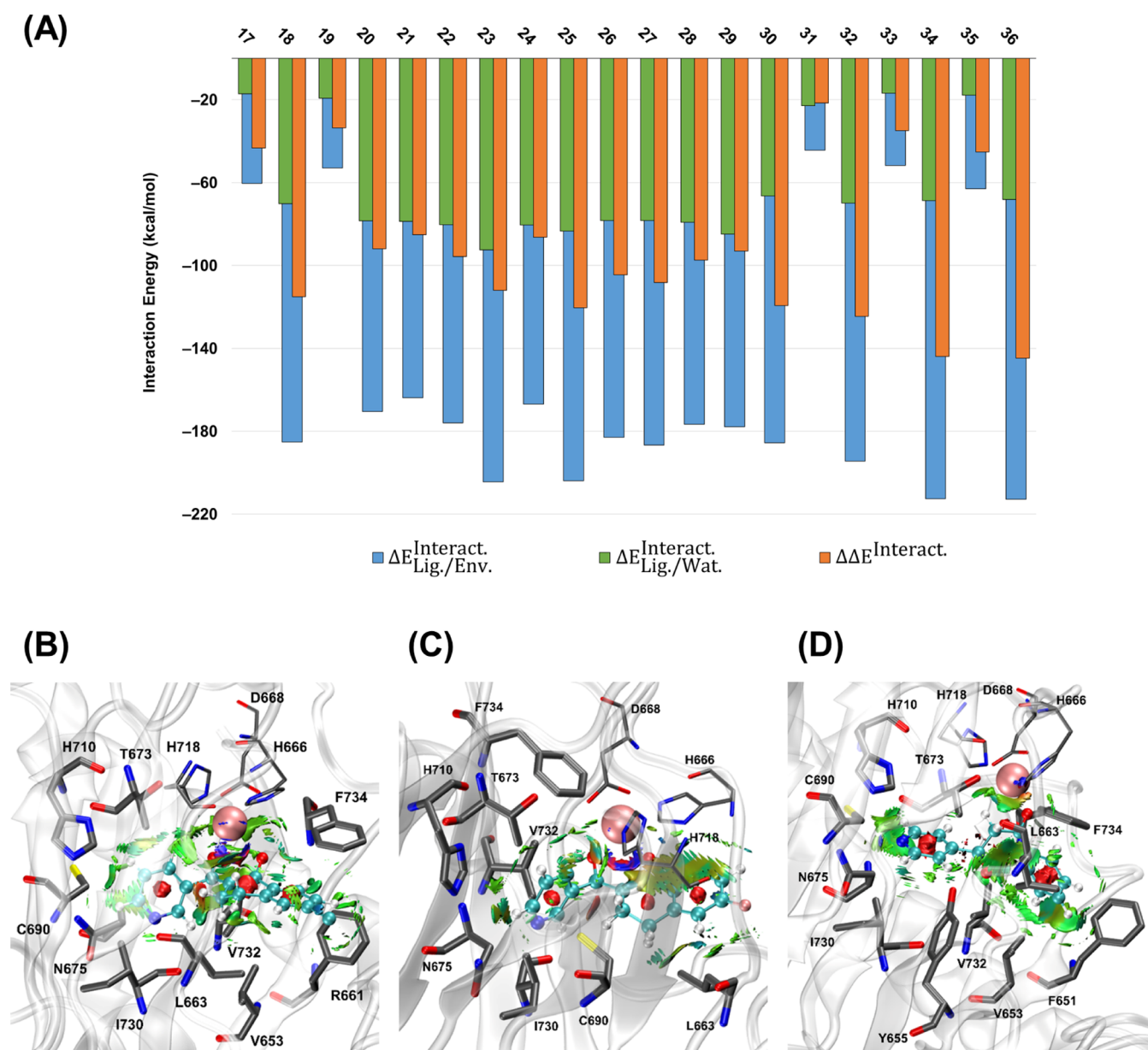
Figure 3. (A) Calculated QM/MM interaction energies ( \text{kcal mol}^{-1} ) for the second set of the studied ligands (ID: 17–36) at the \omega B97X-D/6-31G(d,p) level of theory and AMOEBABio18 force field. The plot of the noncovalent interactions (NCIs) between the ligand and surrounding amino acid residues for (B) cpd27p, (C) cpd26p, and (D) cpd2p. The isosurface cutoff for the NCI is 0.35 au, and the data is plotted in the color range of -0.05 < \text{sign}(\lambda_2)\rho < 0.05 au. Residues H666, D668, and H718 are shown in thin sticks, ligand atoms are in ball and sticks (with different color codes), \text{Fe}^{2+} is in pink vdW sphere, and the surrounding residues with the noncovalent interactions are in thick sticks. Hydrogen atoms are not shown for more clarity.
