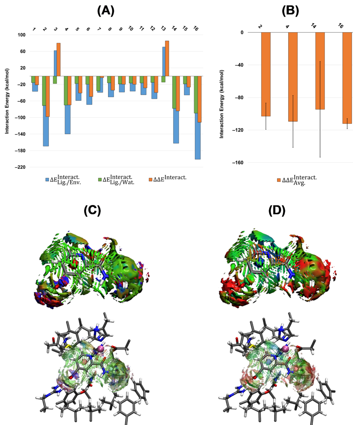
Figure 2. (A) Calculated QM/MM interaction energies ( \text{kcal mol}^{-1} ) for the first set of test compounds (ID: 1–16). (B) Average QM/MM interaction energies ( \Delta \Delta E_{\text{Interact. Avg.}} ) and the standard deviation for the compounds with the most negative interaction energies. All of the calculations are at the \omega B97X-D/6-31G(d,p) level of theory and AMOEBA18 force field. (C) Averaged noncovalent index (aNCI) and (D) thermal fluctuation index (TFI) analyses for cpd12 (ID: 14). The isosurface cutoff for NCI and TFI is 0.4 au, and the data is plotted in the color range of -0.05 < \text{sign}(\lambda_2)\rho < 0.05 au.
