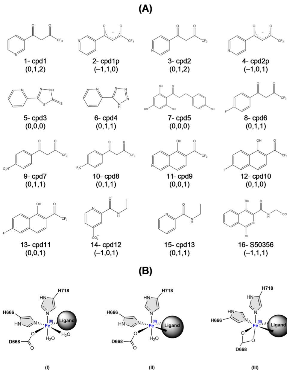
Scheme 1. (A) First Set of Test Compounds a and (B) Possible Coordination Geometries of the Ligands to Fe(II) in the Active Site
