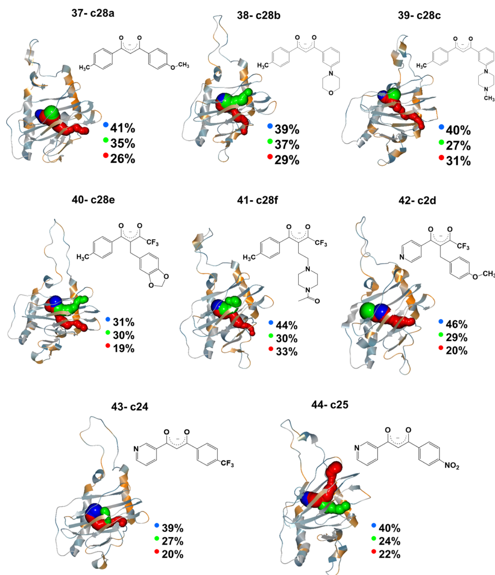
Figure 5. O 2 -transporting tunnels with the largest calculated percentages along the trajectory observed in the third set of lead compounds. The two-dimensional (2D) structure of each ligand is also given next to its tunnel graph. Calculated tunnels are colored in blue, green, and red based on the increase in the tunnel's length. The intersection of the tunnels inside the protein is the active site of the inhibition reaction, but the active site's residues are not shown for more clarity.
