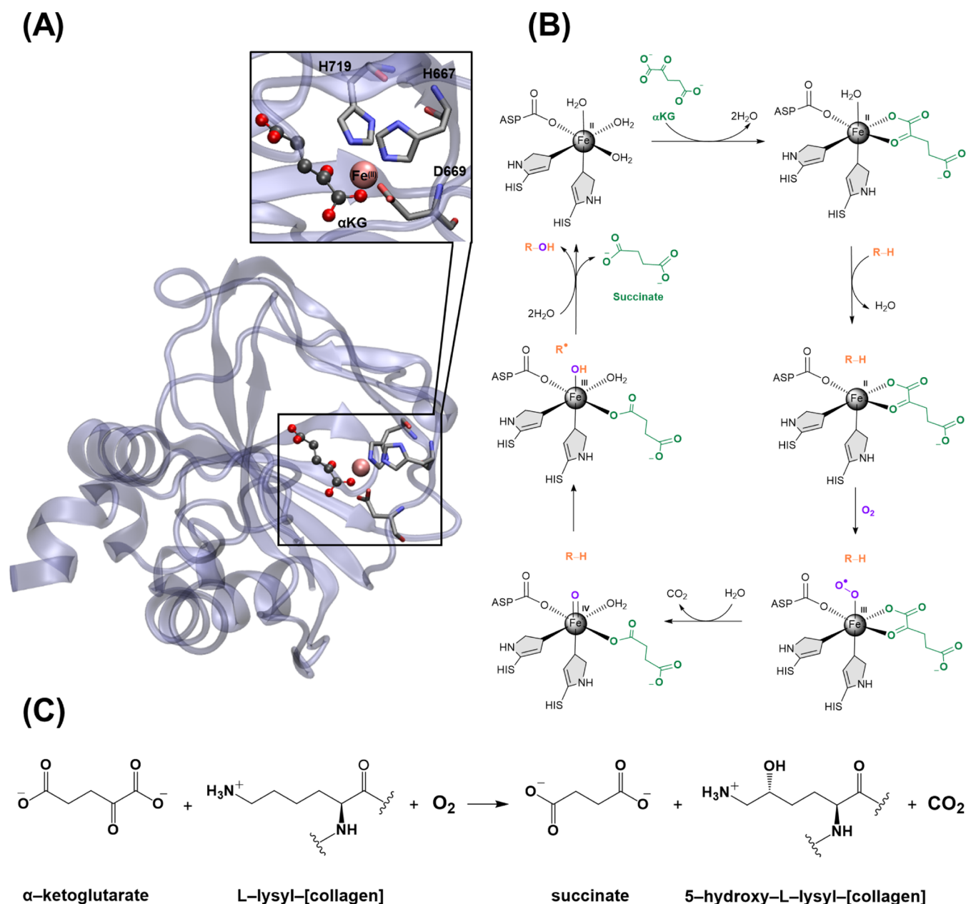
Figure 1. (A) Crystal structure of full-length human lysyl hydroxylase LH3 and its active site complexed with \alpha KG (PDB ID: 6FXK). 24 (B) The general catalytic mechanism of the \alpha KG-dependent hydroxylase superfamily. (C) Hydroxylation of lysine to hydroxylysine by the LH2 in the presence of molecular oxygen.
