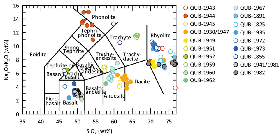
Fig. 3. Total alkali silica plot (following Le Bas et al., 1986) showing glass compositions of tephra reported in this paper. A symbol-based version of this plot is presented in the Supplementary Information (Fig. S1).
