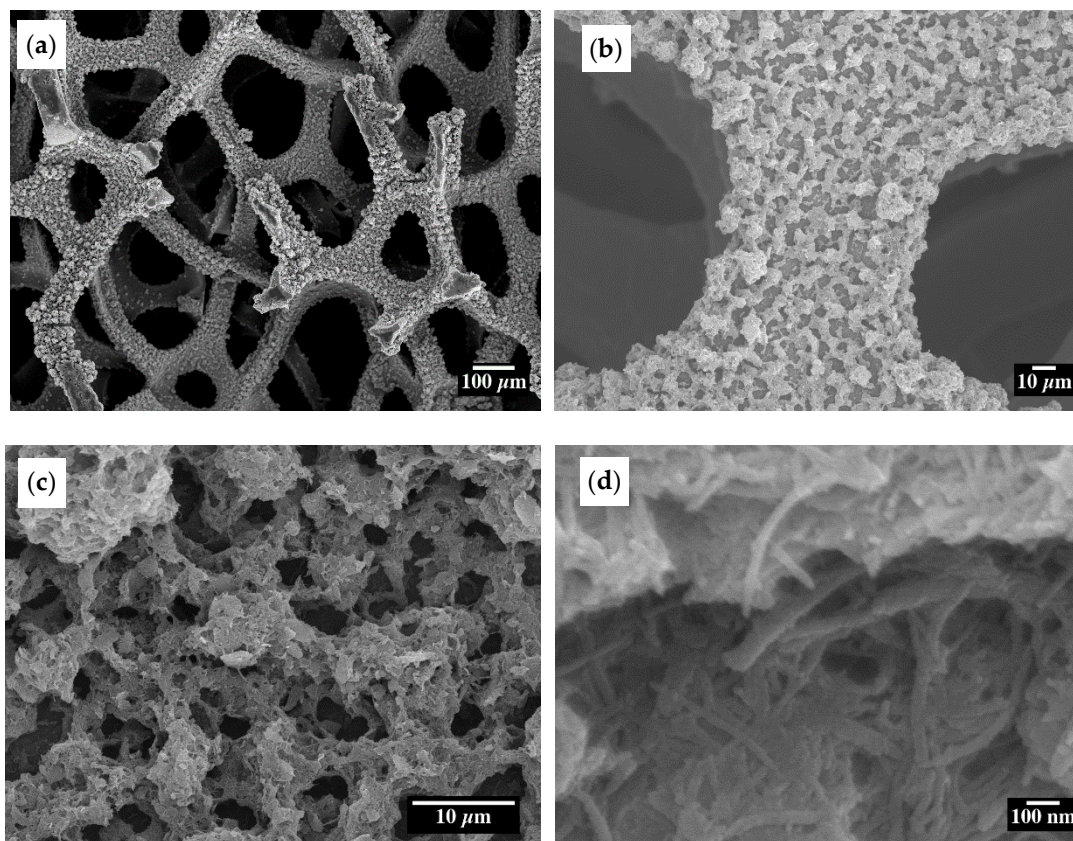
Figure 3. SEM images of the confined \text{SnO}_2 in a CNT at different magnifications (a–c) uniform porous morphology, and (d) dispersed CNT.
