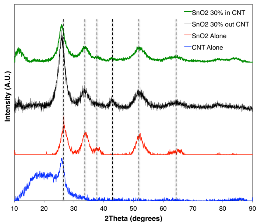
Figure 2. XRD plots for samples with confined and unconfined \text{SnO}_2 in/on a CNT, and also patterns for pure \text{SnO}_2 and a CNT.
