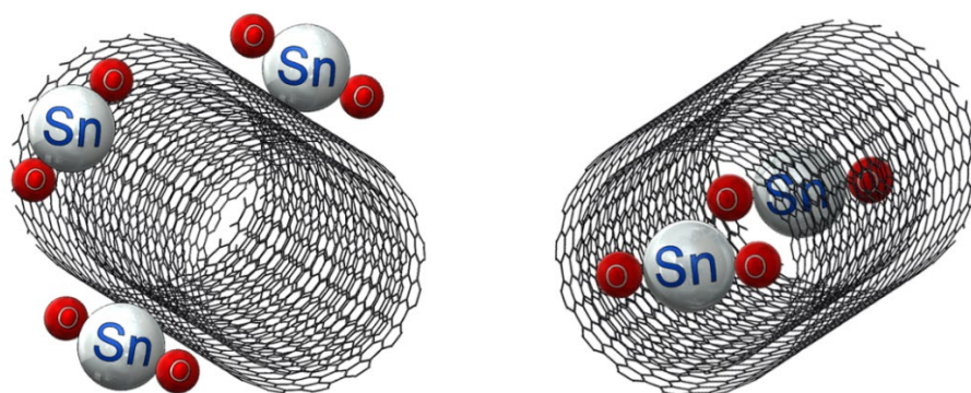
Figure 1. Schematic of unconfined \text{SnO}_2 on a CNT and confined \text{SnO}_2 in a CNT.
