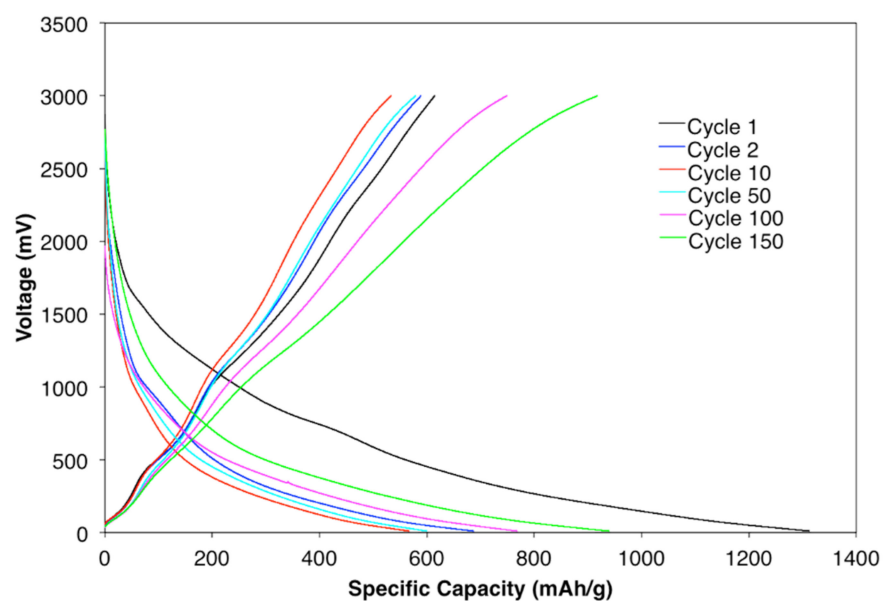
Figure 6. Galvanostatic charge/discharge curves for a sample with 20% confined \text{SnO}_2 in a CNT.
