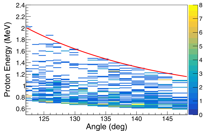
FIG. 1. Energy versus angle of protons in the laboratory frame for the ^{12}\text{Be} + d reaction, gated on a ^{12}\text{Be} ion detected in both the upstream ionization chamber and the downstream S3 telescope. The red curve shows the threshold for the ground state proton.
