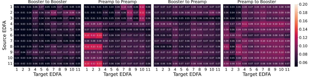
Fig. 3: Transfer Learning MAE matrix of SS-NN model with internal features on random loading. The (i, j) entry corresponds to the TL-based EDFA model, where the i^{\text{th}} and j^{\text{th}} EDFA serve as the source and target models, respectively. EDFA 1-3 are deployed in Open Ireland, while EDFA 4-11 are deployed in COSMOS.
