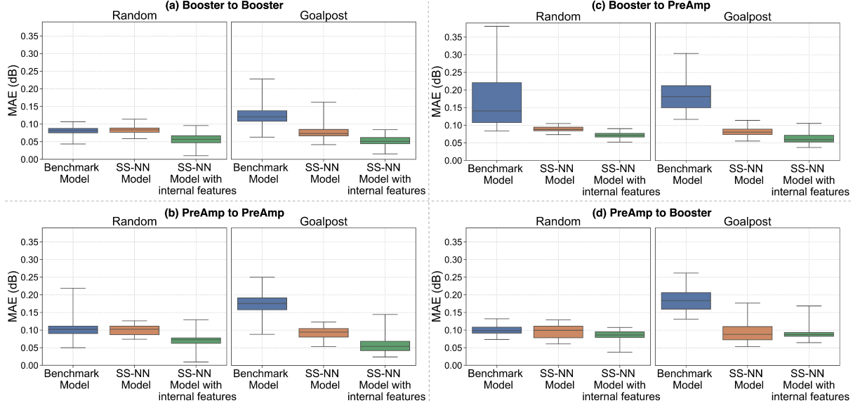
Fig. 2: Boxplot distribution of MAE across 22 EDFAs of (a) Booster to Booster TL, (b) PreAmp to Preamp TL, (c) Booster to Preamp TL and (d) Preamp to Booster TL. The boxes denote the inter-quartile range, and the whiskers denote the min/max.
