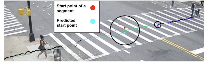
Fig. 6: Demonstration of detection and removal of redundant IDs by the ID Correction algorithm when the tracker assigns 3 IDs to a single pedestrian.
