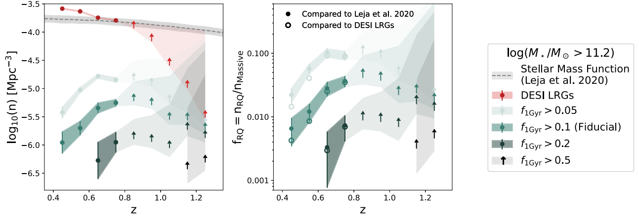
Figure 5. Number densities (left) and fractions (right) of recently quenched galaxies in the mass-complete sample ( \log(M/M_\odot) > 11.2 ; see Section 2.3.2). The dashed line and gray band (left) represent the stellar mass function of similar-mass galaxies (Leja et al. 2020), and the red points show the number density of all LRGs above the mass limit. The light green, medium green, dark green, and black points represent the number densities and fractions of recently quenched galaxies with f_{1\text{ Gyr}} greater than 0.05, 0.1, 0.2, and 0.5, respectively, as compared to the stellar mass function from Leja et al. (2020). In the right panel, the open symbols of the same colors show the fraction of recently quenched galaxies compared to our own massive galaxy number density measurements. Above z = 0.8 , measurements are indicated as lower limits with errors inflated to encapsulate the possibility that all galaxies that were not targeted by DESI meet the selection criterion.
