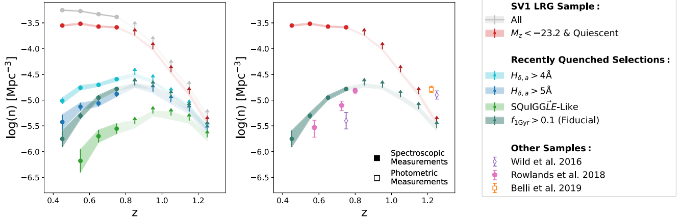
Figure 4. (Left) Number densities within the DESI SV LRG sample (full sample, gray; luminosity-complete and quiescent, red) and a variety of recently quenched selections from the magnitude-limited (see Section 2.3.1) quiescent sample ( H_{\delta,a} > 4 , light blue; H_{\delta,a} > 5 , dark blue; SQuIGGLE SED selection, light green; and f_{1\text{Gyr}} > 0.1 , green). Beyond z \sim 0.8 , we indicate that the measured number densities are lower limits by plotting them as upward-facing arrows. All recently quenched selections show an increasing number density over the redshift range in which we are complete, with varying normalization resulting from the relative restrictiveness of the post-starburst criteria. (Right) Same magnitude-limited LRG and f_{1\text{Gyr}} > 0.1 samples as the left panel, in addition to literature measurements (photometric, open symbols; spectroscopic, filled symbols). All three of the Wild et al. (2016; M_z > 10^{10.8} M_\odot ), Rowlands et al. (2018; M_* > 10^{11} M_\odot ), and Belli et al. (2019; M_* > 10^{10.8} M_\odot ) samples show a trend of increasing number density with redshift, but the normalization differs between the different samples as a result of differing stellar mass limits and selection techniques.
