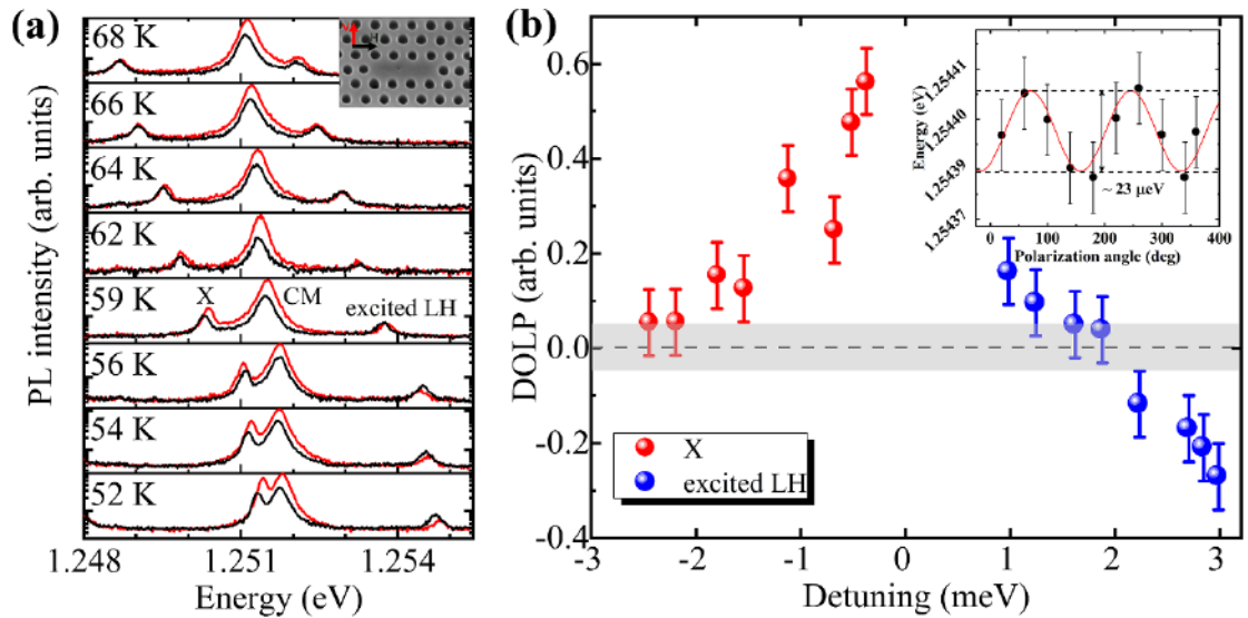
Figure 3. Phonon-assisted coupling examined by the degree of linear polarization (DOLP). (a) \mu PL spectrum resolved in H (black) and V (red) polarizations in the QD-CM detuning range from -3 meV to 3 meV. Inset: H and V polarization with respect to the cavity orientation. (b) DOLP of X and LH as a function of their detuning with respect to CM extracted from a. The black dash line marks the zero-DOLP line, and the grey bar region is the typical DOLP value for bare QDs without the presence of a cavity. Negative DOLP is observed over a much larger \approx 2 meV detuning range, likely due to intrinsic LDOS of the L3 cavity. Detuning is defined as the energy difference with respect to CM. Measurements are with 532 nm CW excitation. Inset: X emission energy as a function of the half-wave plate fast-axis angle, indicative of the fine-structure splitting. The data deviates from a linear energy shift due to temperature drift during the measurement.
