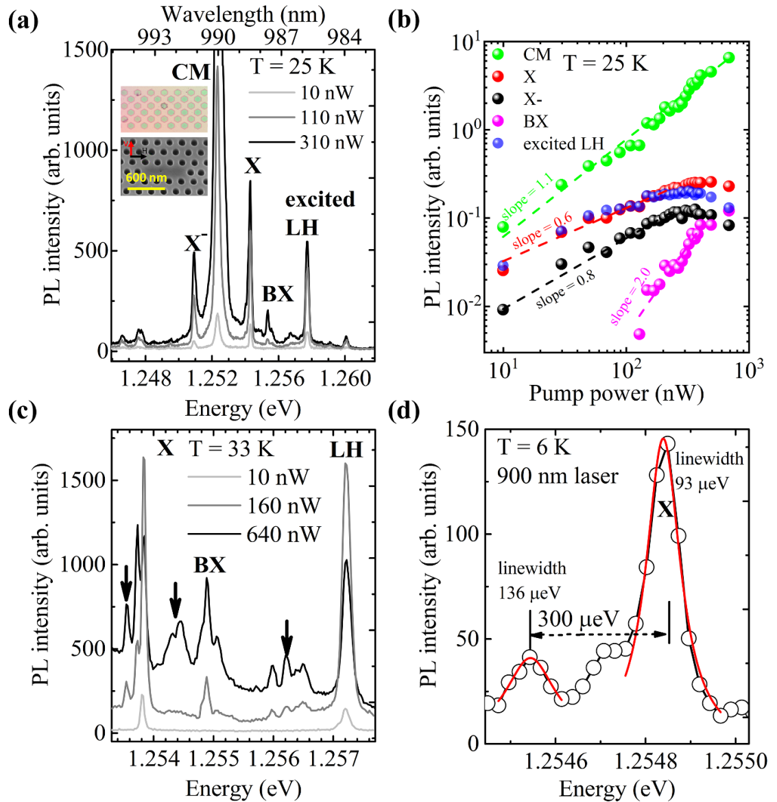
Figure 1. Exciton complexes and dark excitons in single site-controlled InGaAs cavity quantum electrodynamics. (a) \mu PL spectrum of a single pyramidal InGaAs QD-L3 PhC cavity system at 25 K with 532 nm non-resonant pumping at 10 nW, 110 nW, and 310 nW. Inset: an image of the PhC cavity. Scale bar: 600 nm. (b) Integrated \mu PL intensity of different QD exciton species and cavity mode as a function of pump power at 25 K. (c) A zoom-in of the exciton complex species marked by arrows at 33 K (near the X and BX emission) with 532 nm non-resonant pumping at 10 nW, 160 nW, and 640 nW. (d) Sample zoom-in of the peak 300 \mu eV below X emission, at 6 K with 900 nm pumping.
