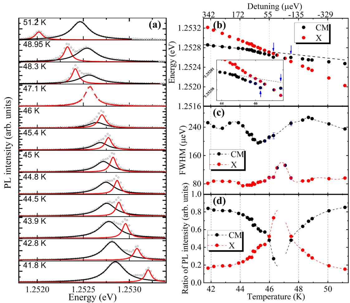
Figure 2. Observations of the coexisting strong-weak coupling regimes probed by high-resolution cryogenic spectroscopy and stepped temperature dependent \mu PL. (a) Temperature-dependent \mu PL traces of CM and X emission. (b) Peak energy of CM and X emission as a function of temperature extracted by spectral Lorentzian fitting of a. The black dashed line indicates the slopes of CM at large X-CM detuning. Inset: zoom-in of the mode crossing. (c) Linewidth of CM and X as a function of temperature. The partial out-of-the-synchronization linewidth averaging supports an intermediate coupling region mediated by phonon scattering, with a collective state emission. (d) Ratio of the integrated CM and X emission intensity as a function of temperature. Half black and red circles near zero detuning are from single Lorentzian fits. Black and red dash lines are guides to the eyes. Measurements are with 900 nm pulsed excitation.
