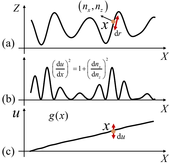
Figure 3. 2D simplification of UV map estimation. We illustrate the isometric relationship between (a) the surface and (c) the UV map. The length of the curve in XZ axis needs to be preserved when mapping to g(x) , i.e., |du| = |dr| = \sqrt{dx^2 + dz^2} (arc length preservation). This relationship can be re-written as (b) a partial differential equation using Equation (6) in terms of its surface normal and the inverse of the spatial derivative of g , i.e., \left(\frac{du}{dx}\right)^2 = 1 + \left(\frac{dn_x}{dn_z}\right)^2 .
