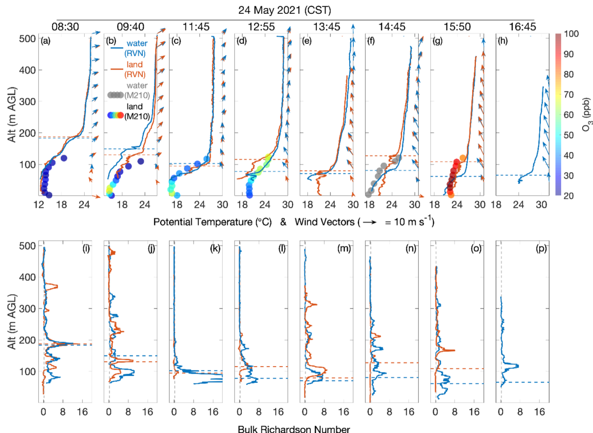
Fig. 7 (a–h) Show q vertical profiles for sets of profiling measurements spaced roughly one hour apart throughout May 24, 2021. Orange and blue solid profiles represent RAVEN profiles measured over land and water, respectively, while M210 flights over land are depicted as q profiles with O_3 colormap (ppb) and M210 flight over water (grey). Dashed lines indicate h_{\max-N^2} . Wind vector profiles are shown at the righthand side of each panel. Arrow direction indicates azimuthal direction. Arrow length is relative to wind speed. (i–p) Show bulk Richardson number vertical profiles, smoothed using a 20 m moving median.
