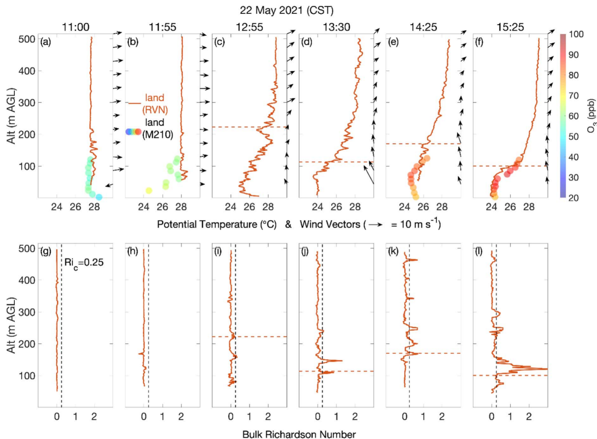
Fig. 6 (a–f) Show q profiles for sets of profiling measurements spaced roughly one hour apart throughout May 22, 2021 (three morning profiles were omitted that had consistent behavior to the 17:00 and 17:55 UTC profiles). Orange lines represent RAAVEN profiles measured over land and M210 flights over land are depicted as q profiles with O_3 colormap (ppb). Circles indicate h_{\max-N^2} . Wind vector profiles are shown at the righthand side of each panel. Arrow direction indicates azimuthal direction. Arrow length is relative to wind speed. (g–l) Show bulk Richardson number profiles, smoothed using a 20 m moving median.
