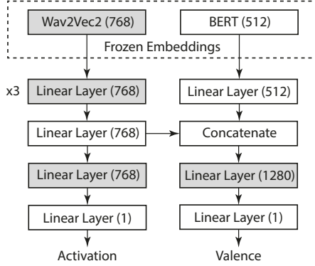
Figure 1: Diagram of the model architecture. All linear layers have LayerNorm applied to their inputs, and all layers in gray have LeakyReLU and Dropout applied. Dropout is also applied to the BERT CLS token.
