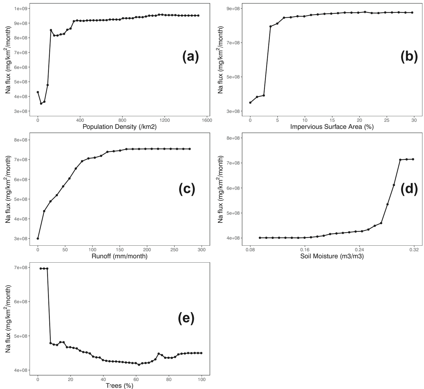
Fig. 3. Partial dependence plots showing variation in monthly riverine sodium flux varies with each individual predictor feature including (a) population density, (b) impervious surface area, (c) runoff, (d) soil moisture, and (e) percent tree cover.
