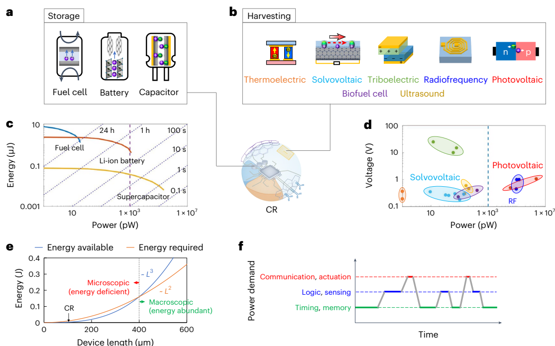
Fig. 2 | Energy harvesting and storage techniques relevant for CRs.
