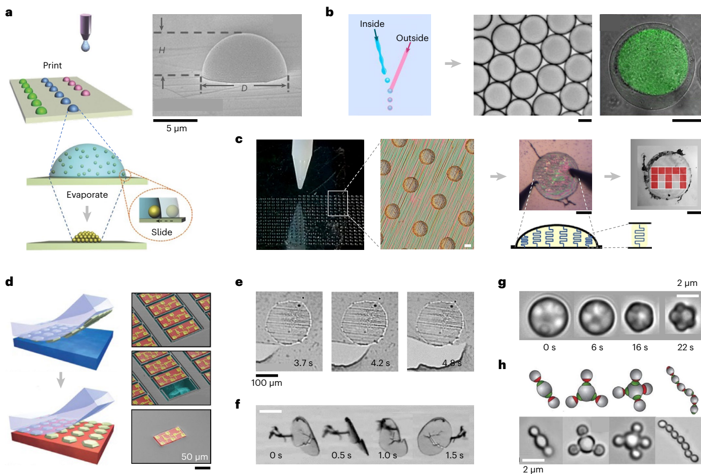
Fig. 3 | Selected examples of device integration relevant for colloidal robotics applications. a , Schematic of the process of assembling inkjet-printed polystyrene beads into aggregated dome-shaped arrays. Inset: scanning electron micrograph (SEM) image of one such printed polystyrene micro-dome 77 . H , height; D , diameter. b , High-throughput in-air microfluidic inkjet printing of micro-suspensions of multiple compositions 51 . Left: schematic of the technique that generates core-shell structures. Middle: spherical particle suspensions viewed via optical microscopy. Right: multi-material (alginate-dextran-tyramine in H_2O ) core-shell particles. Scale bars, 50 \mu m . c , Inkjet printing of CR particles consisting of graphene-encapsulated memristor arrays. Left: optical image (inset: micrograph) of the printed microparticles. Middle: top view of the electrical characterization of a single microparticle (after solution lift-off and recapture). Bottom-right inset: schematic cross-section of the vertical memristor array. Top right: a 15-bit microparticle memristor array written via electronic probes. An 'M'-shaped vertical conductivity map (red, ON; clear, OFF) overlaid on top of the microparticle tested. Scale bars, 50 \mu m (ref. 10).
