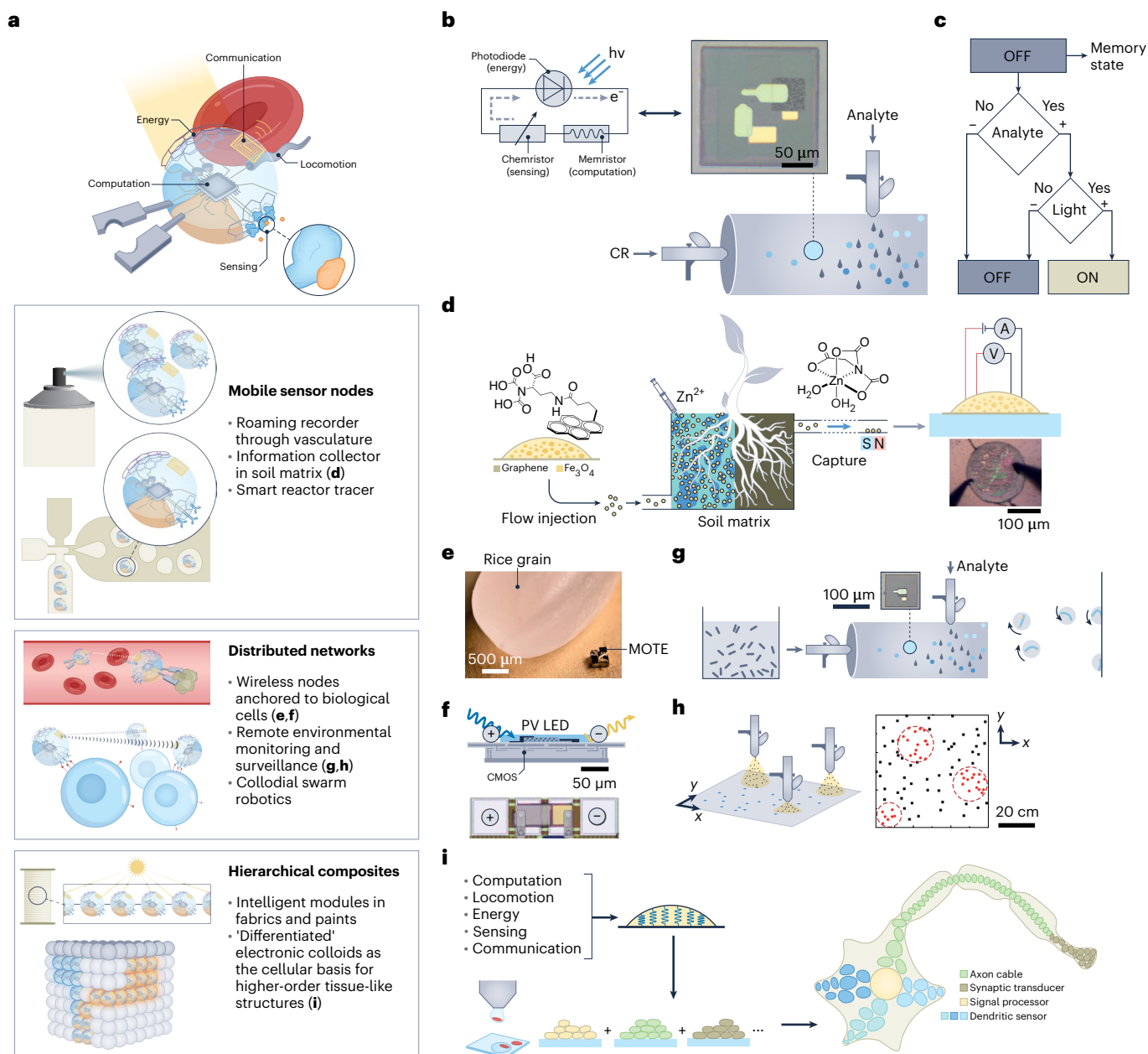
Fig. 1 | Concepts and prototypes of CRs. a , Schematic of a CR. b , Schematic of an early CR prototype being used for analyte and light detection inside a vapour chamber 9 . Left: electrical circuit diagram of the CR. The photodiode converts light into current, which turns on the memristor if, and only if, the chemristor detects a prescribed analyte. Right: top-view optical micrograph of the CR used 9 . c , Block diagram of the CR summarizing the combinational logic. The initial memory state OFF changes to ON only in the presence of both chemical and light signals 9 . d , Schematic of the deployment of surface-functionalized colloidal electronic microparticles as chemical probes to detect and record the presence of various species, such as Zn^{2+} ions in the soil matrix. Symbols S and N represent the south and north poles of the externally applied magnetic field, respectively. Inset: optical micrograph of the colloidal electronic particle during electrical readout 10 . e , A laser-powered 0.04 mm 3 16 nW wireless sensor microscale opto-electronically transduced electrode (MOTE) with integrated central processing and optical communication capable of accurate cellular temperature measurement in vitro 15 .
