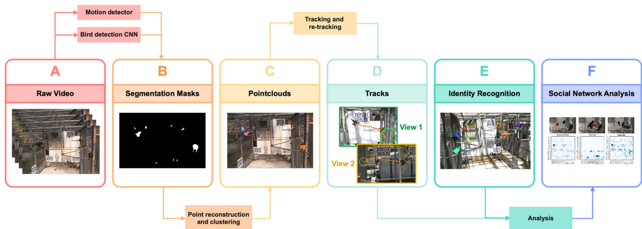
Fig. 1 Full pipeline for cowbird tracking and recognition. A A synchronized set of raw videos from multiple views are processed in a frame-by-frame manner. B Segmentation masks of bird instances are obtained using a Mask R-CNN network and background subtraction. C Pointclouds are reconstructed by multi-view matching, triangulation, and clustering. D Tracking, which is implemented using a Lagrangian
