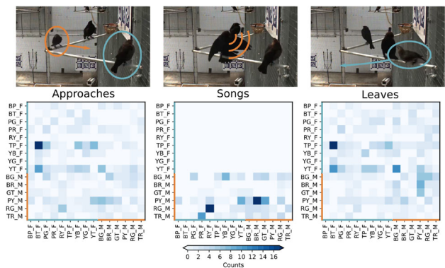
Fig. 8 Pairwise interactions. Approaches, songs, and leave interactions occur frequently between individuals in the aviary. Each matrix shows the frequency of interactions for each pair of individuals. The bird performing the action is shown on the left axis (the approaching, singing, or leaving bird) and the target or recipient of the action is shown along the bottom axis (the approached, receiving, or remaining bird). Orange indicates males and blue indicates females. Approaches and leaves show relative movement between individuals and reveal differences in activity levels and dominance (see Sect. 6.3). We also observed six pair bonds between males and females, which are defined whenever a female receives more than 50% of songs from a single male (Anderson et al., 2021)
