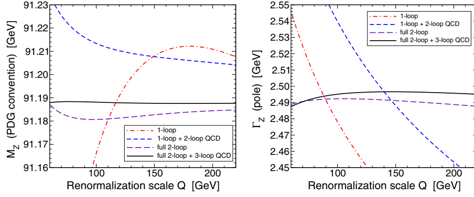
FIG. 2. The Z boson mass in the PDG-convention M_Z^{\text{PDG}} (left) and the width \Gamma_Z (right), obtained from the calculated complex pole mass s_{\text{pole}}^Z , as a function of the renormalization scale Q . The different lines show various approximations as labeled. The \overline{\text{MS}} input parameters are as given in Eq. (1.17), which provide for M_Z^{\text{PDG}} = 91.1876 GeV when calculated at the renormalization scale Q = 160 GeV using the full two-loop plus three-loop QCD approximation.
