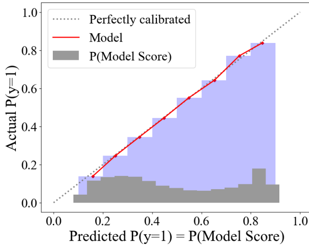
(a) Reliability diagram (for accuracy)
