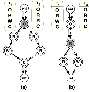
Fig. 4: Paths corresponding to traces and the location of the divergence point (shaded gray). For the same traces, the location of the divergence point changes based on the specification.
