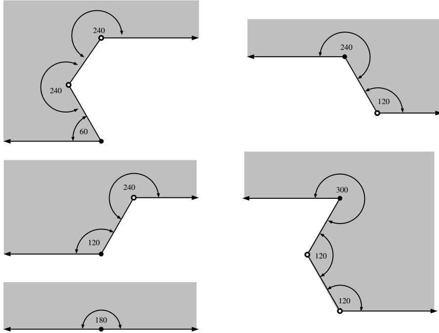
Figure 16: The five cases for assigning image angles and associated vertices. In each case the black indicates the image of the original vertex and the white dots the new associated vertices. These arcs illustrate small subarcs of the 60^\circ -polygon P' . The associated vertices map to 180^\circ vertices that we add to the edges of P .
