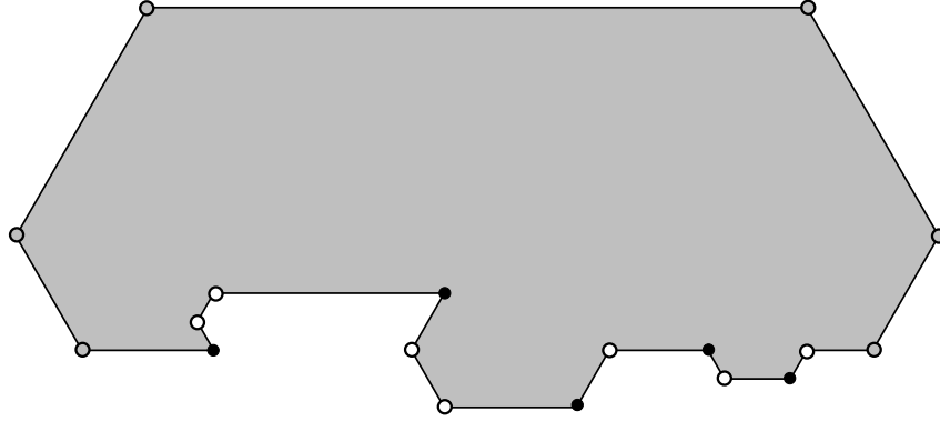
Figure 17: The 60°-polygon P' . The six gray points were added at the beginning, the black points are the images of the original vertices and the white points are the associated vertices.
