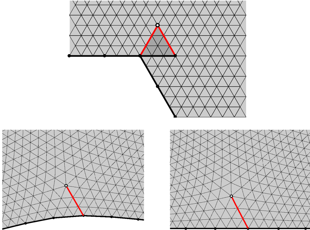
Figure 14: The Riemann surface R can be conformally mapped to a slit domain \Omega by a branch of z^{6/7} . This map is followed by a conformal map to the upper half-plane that bends the the straight slit to an analytic arc (but it looks quite straight; the tangent directions only change by about 1^\circ along the arc).
