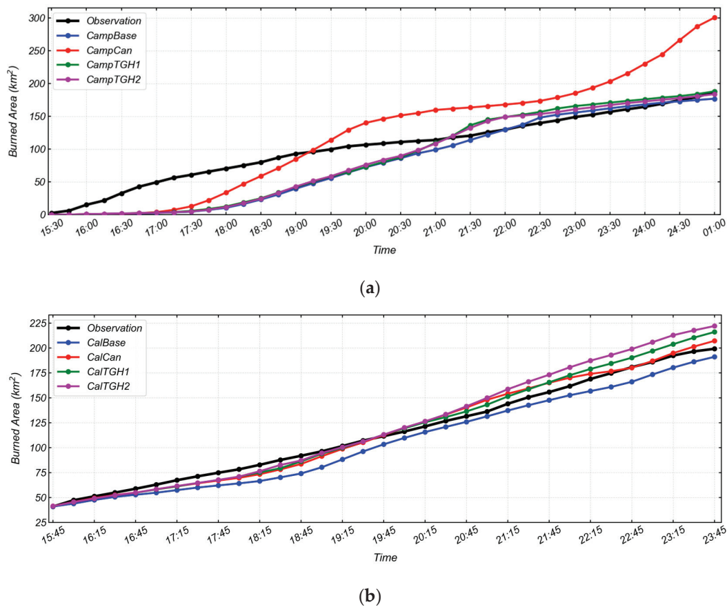
Figure 13. Comparison of the burned area from the simulations and NEXRAD-derived fire perimeters for (a) Camp Fire and (b) Caldor Fire. Abbreviations are based on Table 1.
