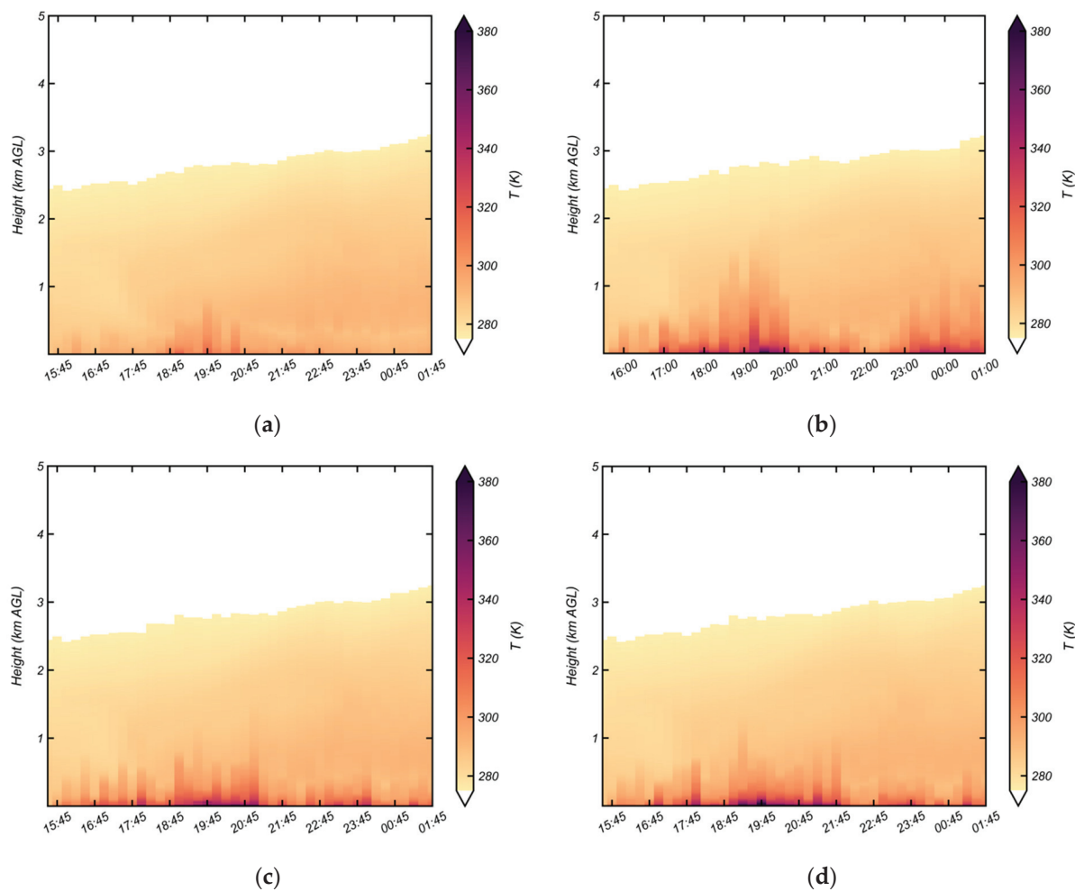
Figure 8. Time height plots of the maximum simulated temperature (T) over the simulation domain for the Camp Fire (a) CampBase, (b) CampCan, (c) CampTGH1, and (d) CampTGH2 cases. Abbreviations are based on Table 1.
