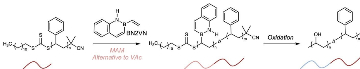
Scheme 1. This work: BN2VN, a more activated monomer (MAM), as an alternative to vinyl acetate (VAc) for the synthesis of vinyl alcohol block copolymers.
