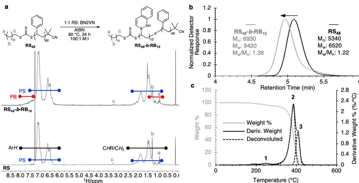
Figure 4. (a) The chain extension of RS 48 to RS 48 - b-RB 10 was successful with retention of the trithiocarbonate end group by 1 H NMR. (b) Unimodal GPC traces show a decrease in retention time. (c) Overlay of TGA (weight % b) and deconvoluted TGA curves (dashed) using Igor 8 multi-peak function with fitted ExpModGauss peak type (gray, dashed) shows three major pyrolysis events (assigned end-group, PS block, and PBN2VN block).
