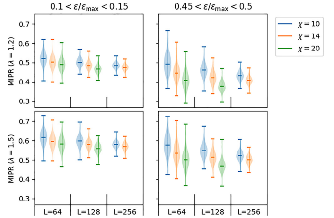
FIG. 22. Violin plots comparing many-body inverse participation ratio across system sizes.
