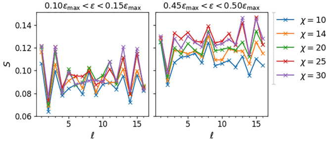
FIG. 5. Single-cut entropy by cut location (i.e., distance from the nearest end point) for strong disorder, \lambda = 3.5 , at L = 64 . The entropy has evidently saturated by \chi = 30 for the different cuts and energies under consideration, and it remains low moving into the bulk, as is generally expected for the area-law behavior of localized states.
