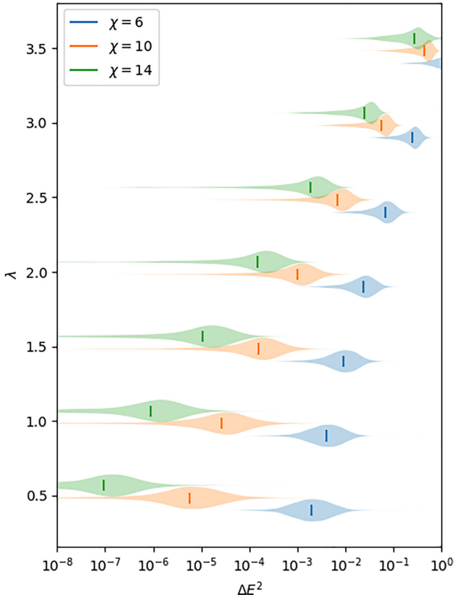
FIG. 14. The distribution of energy errors at several (smaller) bond dimensions, given system size L = 128 , for tests sampling the full spectra of systems with \lambda \in \{0.5, 1.0, 1.5, 2.0, 2.5, 3.0, 3.5\} .
