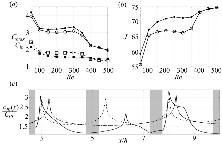
Fig. 12. Model and CFD results for the staggered arrangement. (a) Comparison of CFD results for C_{max} (solid dots) and C_{osc} (solid squares) with model predictions for C_{max} (open circles) and C_{osc} (open squares). (b) Comparison of CFD (solid dots) and model (open circles) predictions for J . (c) Comparison of c_m(x) produced by the reduced model (dashed line) and CFD (solid line) for the staggered arrangement at Re = 300 . The dashed-dotted line shows reduced model results obtained using \lambda = 10 mm.
