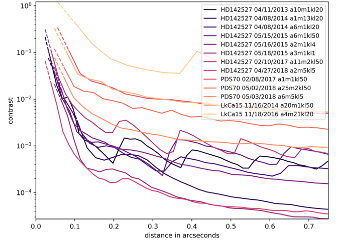
Figure 6. Throughput-corrected 5\sigma contrast curves of all epochs for continuum false planet optimized pyKLIP reductions of the three previously reported GApIPlanetS companion and companion candidate-hosts: HD 142527 (seven epochs), PDS 70 (three epochs), and LkCa 15 (two epochs). Throughput was computed as described in the text, with a correction for the small number of independent noise samples near the star following Mawet et al. (2014). Solid curves indicate regions where throughput-corrected contrast was computed directly. The curves are also projected inward from the innermost throughput measurement to the inner working angle, and this extrapolated region is indicated with a dashed line.
