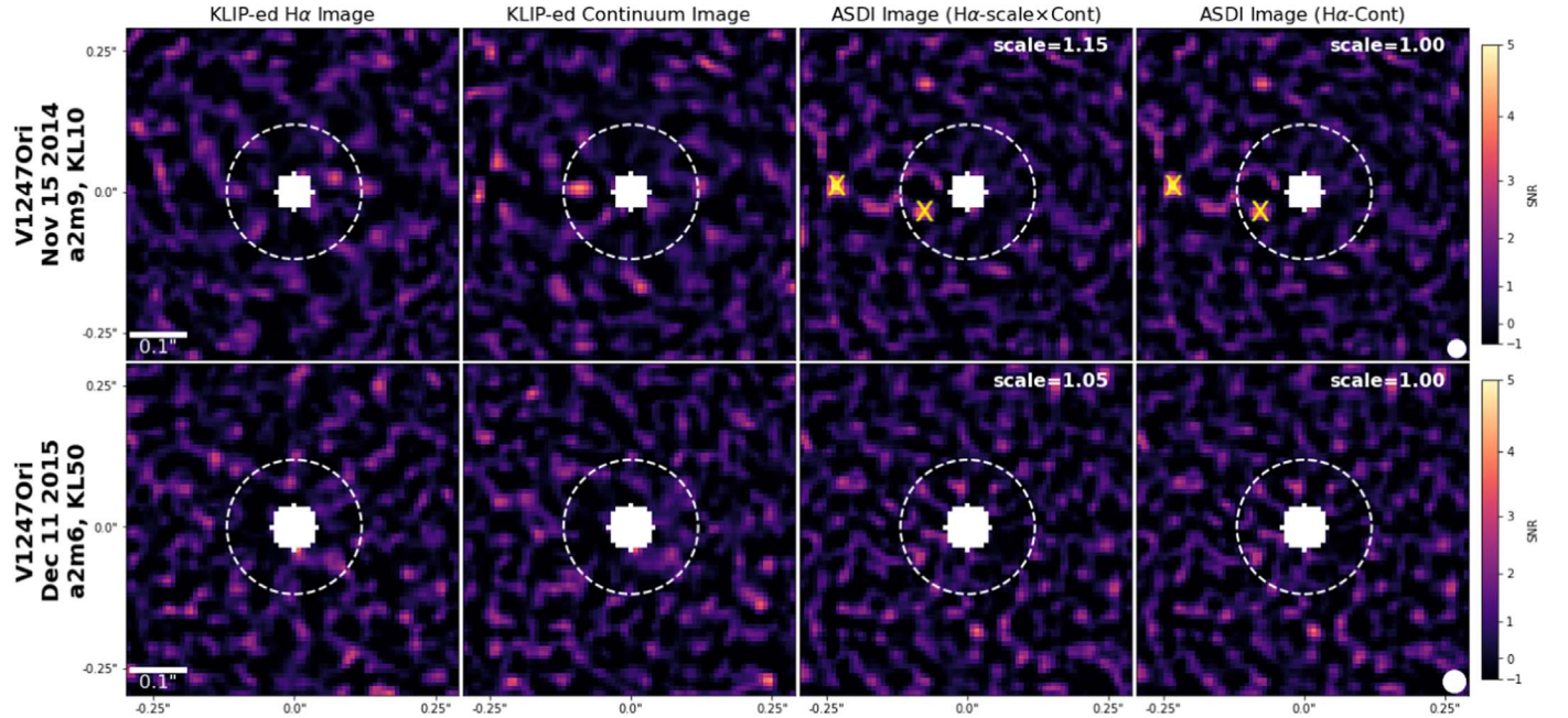
Figure 27. Final KLIPed H\alpha (left), Continuum (middle left), stellar H\alpha /continuum-scaled ASDI (middle right), and 1:1 scaled ASDI (right) imagery for both V1247 Ori epochs. pyKLIP reduction parameters (indicated in the text labels to the left of each image panel) have been optimized for recovery of false continuum planets injected between the IWA and control radius, as described in detail in the text. The AO control radius of the images is indicated with a white dashed circle.
