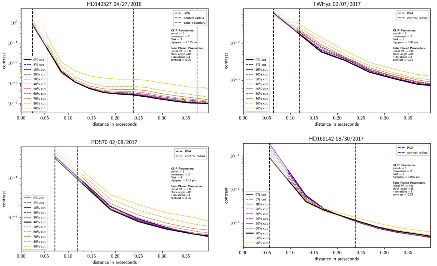
Figure 3. A representative sample of contrast curves used to cull GAPlanetS data sets before KLIP optimization. Each of our four classifications is represented here, namely (clockwise from upper left: clustered, sequential, turnover, and down-and-up). Each colored line represents the post-KLIP contrast achieved by culling different proportions (0%, 5%, 10%, 20%, 30%, 40%, 50%, 60%, 70%, 80%, and 90%) of the lowest-quality images from the sequence, where the FWHM of a Moffat fit to the central star (for unsaturated data) or ghost (for saturated data) is used as a proxy for image quality. The curve is extrapolated inward to the inner working angle following the slope of the two closest points at which throughput was computed. The curves are given higher transparency in this extrapolated region. Curves were computed with a standard set of KLIP parameters (annuli = 5, movement = 2), and are shown here for 10 KL modes (though 5, 10, 20, and 50 mode reductions were also generated and compared before making a final choice). The optimal cut was determined by eye, prioritizing achieved contrast inside of the AO control radius (though several concerns were balanced, as described in the text). Plots for all GAPlanetS data sets are available as a figure set (39 images).
