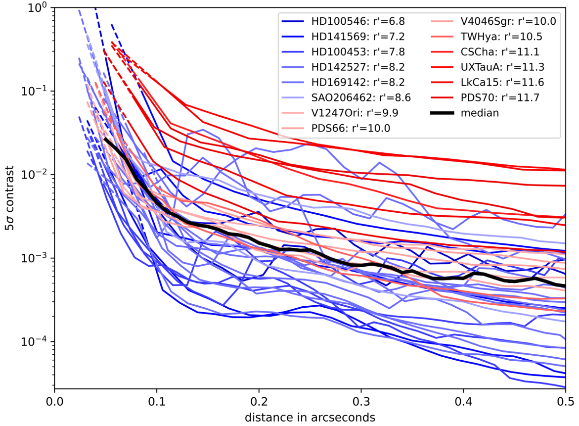
Figure 19. Contrast curves for all GAp PlanetS datasets analyzed in this work. These curves were generated following our conservative survey methodology of optimizing on false continuum planets. Curves are colored by the r' -band magnitude of the star. While the specific contrast achieved for a given target varies widely with seeing, it is also a strong function of r' -band magnitude.
