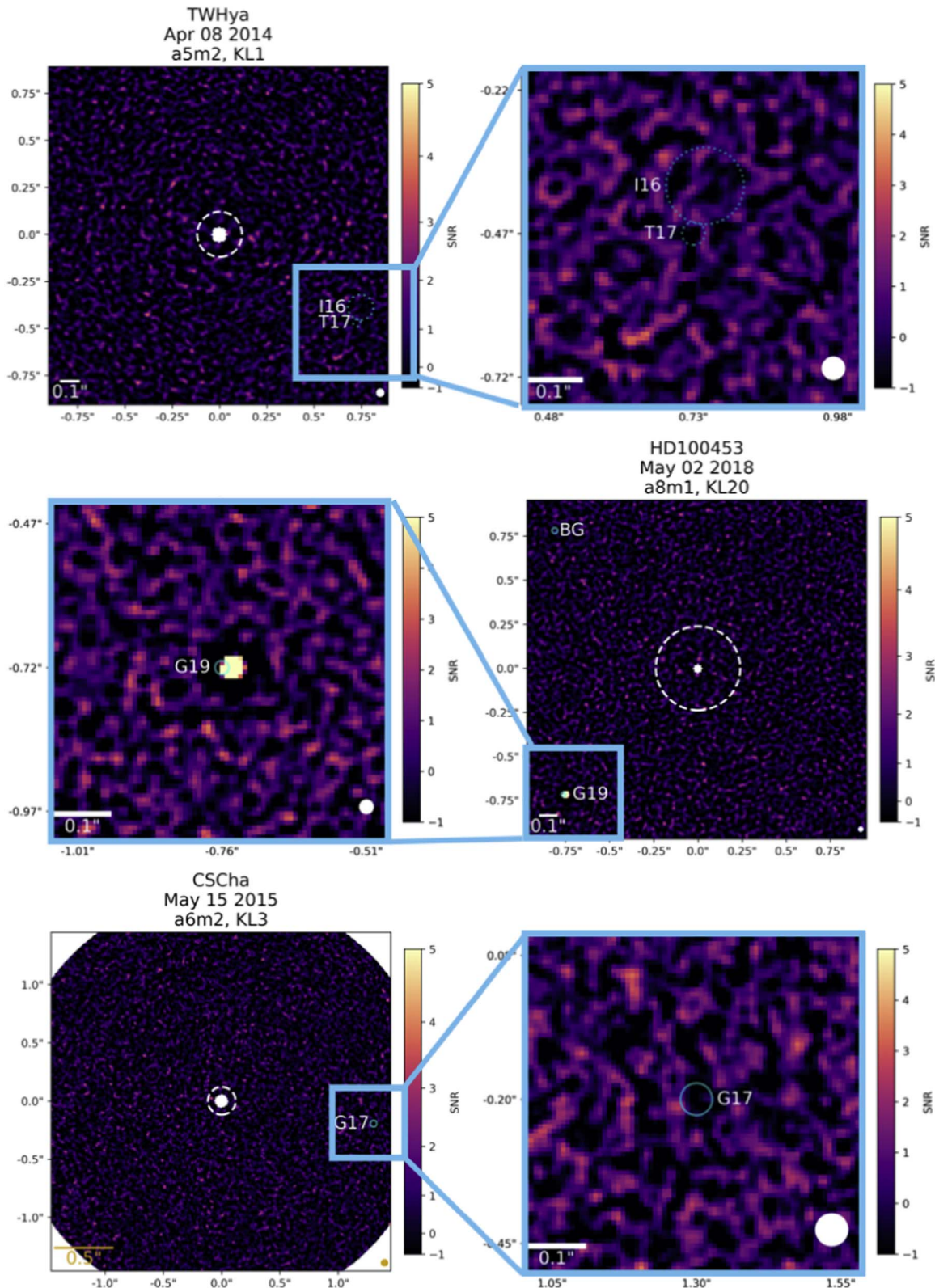
Figure 15. Wide-field and narrow-field views of the 1:1 scaled ASDI reduction from the highest-contrast epoch for all three GAp PlanetS targets with known wide companions (CS Cha B, HD 100453 B) and companion candidates (TW Hya). No clear H \alpha excess signal is present at the location of the wide TW Hya candidate(s) reported in Ilee et al. (2022; “l16”) or Tsukagoshi et al. (2019; “T17”), nor is it apparent from the known, highly embedded CS Cha B companion (“G17,” Ginski et al. 2018). H \alpha excess is, however, apparent from the HD 100453 B companion at a location consistent with its reported position in 2019 (Gonzalez et al. 2020; “G19”).
