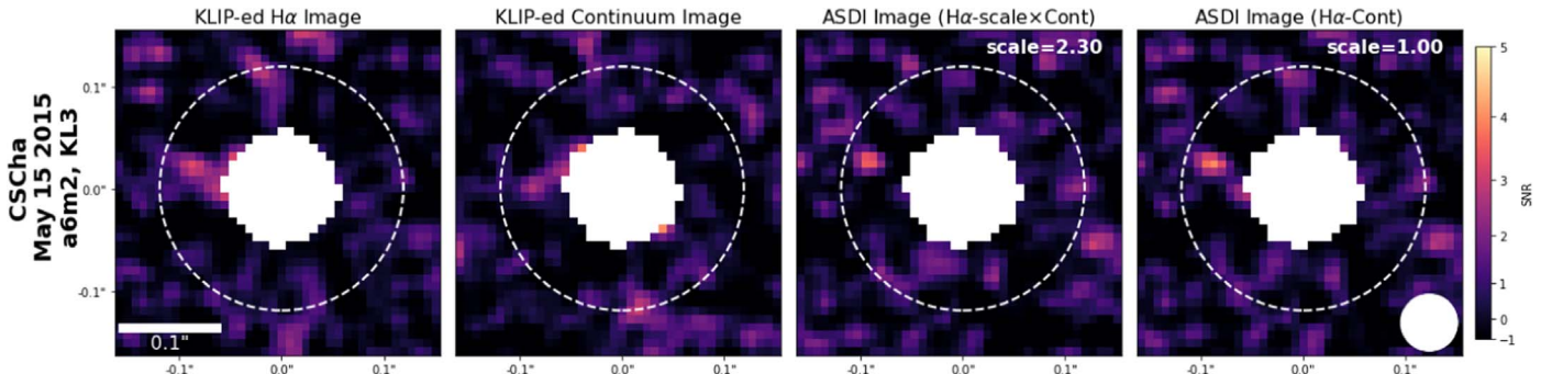
Figure 12. Final KLIPed H \alpha (left), Continuum (middle left), stellar H \alpha /continuum-scaled ASDI (middle right), and 1:1 scaled ASDI (right) imagery for the single GAp PlanetS CS cha epoch. The new candidate companion, CS Cha “c” is apparent to the east of the star in H \alpha and SDI imagery.
