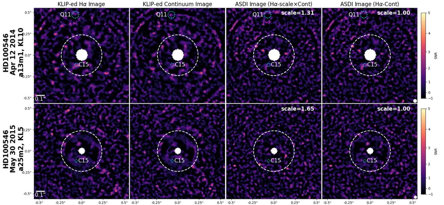
Figure 20. Final KLIPed \text{H}\alpha (left), Continuum (middle left), stellar \text{H}\alpha /continuum-scaled ASDI (middle right) and 1:1 scaled ASDI (right) imagery for both HD 100546 epochs. pyKLIP reduction parameters (indicated in the text labels to the left of each image panel) have been optimized for recovery of false continuum planets injected between the IWA and control radius, as described in detail in the text. The AO control radius of the images is indicated with a white dashed circle. The Currie et al. (2015) and Quanz et al. (2013) planet candidate locations at the original detection epochs are marked with dashed cyan circles labeled “C15” and “Q11,” respectively
