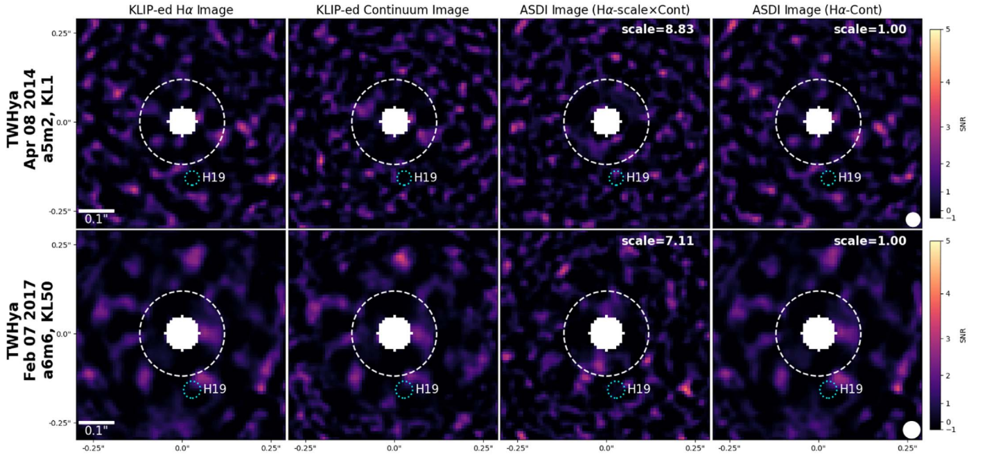
Figure 22. Final KLIPed H\alpha (left), Continuum (middle left), stellar H\alpha /continuum-scaled ASDI (middle right), and 1:1 scaled ASDI (right) imagery for both TW Hya epochs. pyKLIP reduction parameters (indicated in the text labels to the left of each image panel) have been optimized for recovery of false continuum planets injected between the IWA and control radius, as described in detail in the text. The AO control radius of the images is indicated with a white dashed circle. The Huélamo et al. (2022) point-source candidate (a suspected artifact according to the authors) is marked with a dashed cyan circle labeled “H19.”
