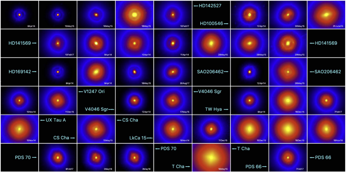
Figure 1. Median combinations of the images in each GApIPlanetS image sequence, normalized to 1 by dividing by the peak pixel and arranged from brightest to faintest r' band magnitude. The extreme variability in the PSF between objects and among images of the same object acquired on different nights is apparent in the variable size of the PSFs. The VisAO PSF is highly dependent on weather conditions.
