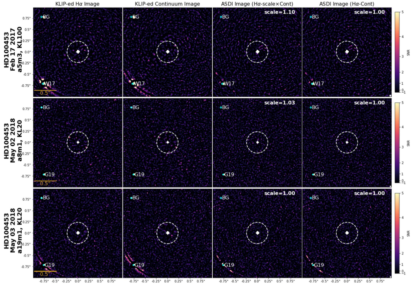
Figure 23. Final KLIPed H\alpha (left), Continuum (middle left), stellar H\alpha /continuum-scaled ASDI (middle right), and 1:1 scaled ASDI (right) imagery for all three HD 100453 epochs. pyKLIP reduction parameters (indicated in the text labels to the left of each image panel) have been optimized for recovery of false continuum planets injected between the IWA and control radius, as described in detail in the text. The AO control radius of the images is indicated with a white dashed circle. The companion HD 100453 B, is clearly visible in the lower left of each image panel, and its locations from Wagner et al. (2018b) and Gonzalez et al. (2020) are marked with cyan circles labeled “W17” and “G19,” respectively. A known background star lies in the upper left-hand corner of each H\alpha and Continuum image (except in the 2018 May 2 epoch, when it is saturated and therefore not completely removed through SDI subtraction), but is absent in the SDI imagery because it is not actively accreting.
