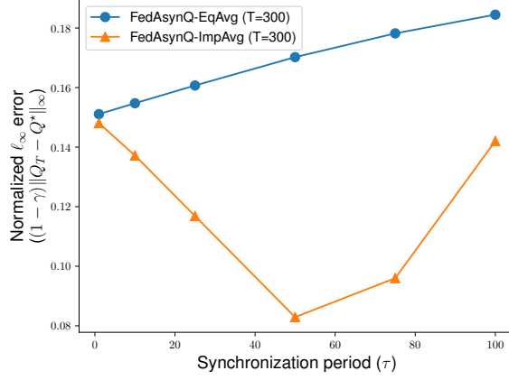
Figure 5. The normalized \ell_\infty error of the Q-estimates (1 - \gamma)\|Q_T - Q^*\|_\infty with respect to the synchronization period \tau = 1, 10, 25, 50, 75, 100 for both FedAsynQ-EqAvg and FedAsynQ-ImAvg, with K = 20 and T = 300 .
