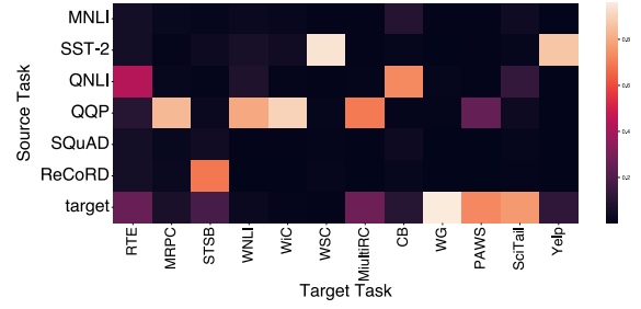
Figure 6: Attention visualizations of ATTEMPT.
