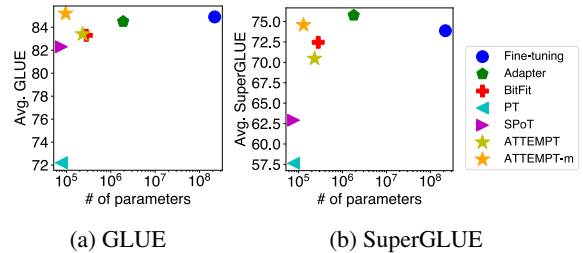
Figure 3: Parameter-efficiency and average scores. We use T5-base for all of the models.
