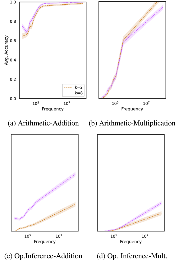
Figure 8: The GPT-J-6B accuracy on arithmetic and operator inference tasks , with k shots. The average accuracy ( y -axis) of the binned instances is highly correlated with their co-occurrences term frequencies \omega_{\{x_1, x_2\}} in the pretraining corpus ( x -axis).
