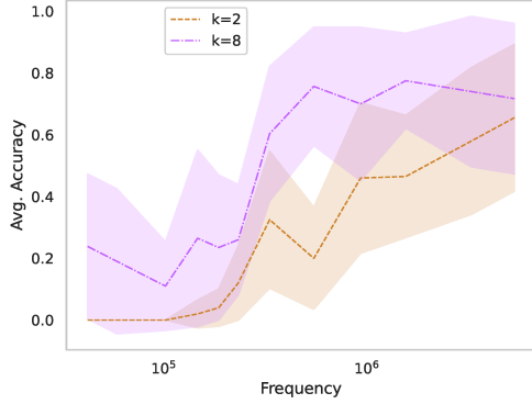
Figure 4: GPT-J-6B performance on Year→Month: Interpolation lines show the correlation between the average accuracy and the \omega_{\{x_1, x_2\}} ( k is number of shots).
