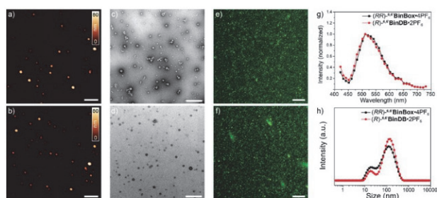
Figure 5. Morphological characterization of the aggregates of (R)- 6,6 BinDB-2PF 6 and (RR)- 6,6 BinBox-4PF 6 formed in 90:10 H 2 O/DMF. a,b) AFM of drop-casted samples on mica of a) (R)- 6,6 BinDB-2PF 6 and b) (RR)- 6,6 BinBox-4PF 6 . Scale bars are 500 nm. c,d) TEM of negatively-stained samples of c) (R)- 6,6 BinDB-2PF 6 and d) (RR)- 6,6 BinBox-4PF 6 . Scale bars are 500 nm. e,f) CLSM of liquid samples of a) (R)- 6,6 BinDB-2PF 6 and b) (RR)- 6,6 BinBox-4PF 6 . Scale bars are 10 μm. g) Extracted emission spectra from confocal-laser scanning experiments. h) DLS of aggregates.
