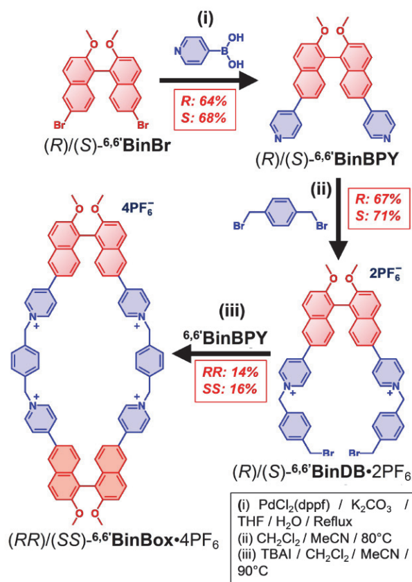
Scheme 1. Synthesis of the axially chiral binaphthyl-based cyclophanes (RR)/(SS)- ^{6,6} BinBox-4PF 6 .
