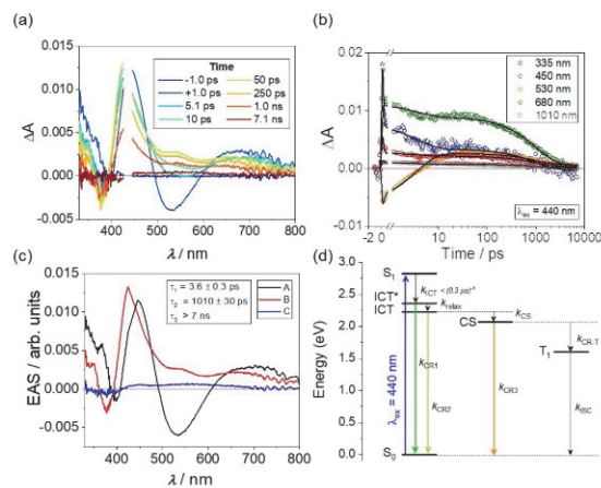
Figure 7. Transient absorption (TA) data for 6,6 BinBox-4PF 6 in a H 2 O/DMF (90:10) mixture excited at 440 nm. a) Spectra at selected time delays. b) Kinetic Fits. c) Evolution-associated spectra after photo-excitation and time constants d) State diagram showing competitive decay pathways: intramolecular charge transfer (ICT), structural/vibrational relaxation (relax), radiative charge recombination (CR1, CR2, and CR3), charge separation (CS), charge recombination to the triplet state (CR-T), and intersystem crossing (ISC). Aggregation causes relaxation to decay biexponentially.
