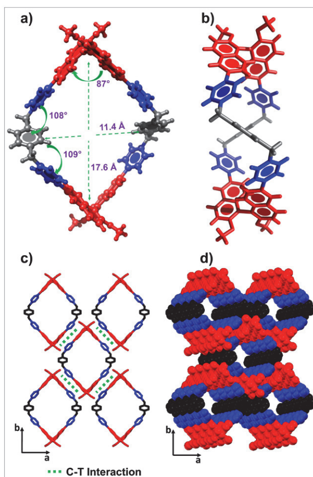
Figure 1. a) Top view and b) side-on view of the X-ray crystal structure of (SS)- ^{6,6} BinBox-4PF 6 showing a square-like and a figure-eight-like structure, respectively. Along the c -axis, the packing of the solid-state structure of (SS)- ^{6,6} BinBox-4PF 6 displays c) CT interactions between the pyridinium units and the binaphthyl moieties and exhibits d) a tubular superstructure.
