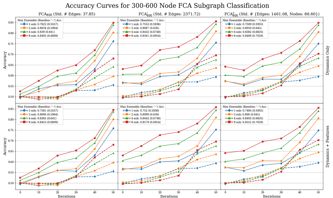
Figure 7. Accuracy curves for predicting synchronization of 5-color FCA on 600-node graphs from dynamics observed from k \in \{1, 2, 4, 8\} subgraphs of 30 nodes. See the caption of Fig. 6 for details.
