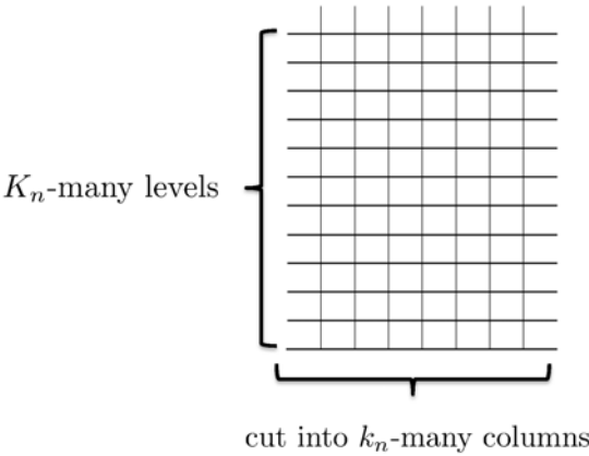
Figure 1. The tower \mathcal{T}_n .
