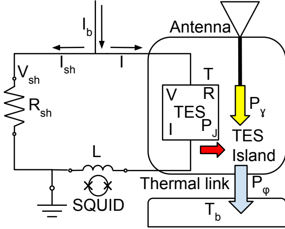
Figure 1. Electrothermal diagram of a TES bolometer. A constant bias current ( I_b ) flows through the TES and a shunt resistor ( R_{sh} \ll R ). The circuit keeps the TES voltage ( V ) nearly constant; therefore, a change in TES resistance ( R ) leads to a change in TES current ( I ). Changes in I are measured with a superconducting quantum interference device (SQUID) connected in series with the TES. Optical power ( P_\gamma ), coupled to the TES bolometer through the antenna, heats the TES island, causing a change in R and hence a current signal measured by the SQUID. At equilibrium, the TES operates on its superconducting transition at temperature T_c , and the sum of the bias power ( P_J ) and P_\gamma dissipated on the island equals the power ( P_\phi ) transported to the bath (at temperature T_b ) by phonons. The interaction between the electrical circuit biasing the TES and the thermal circuit controlling the power flow across the TES island to the bath forms the electrothermal model that governs the TES detector behavior. The coupling between these two systems is determined by the design and intrinsic properties of TES superconducting film, as well as the TES island geometry and its material properties.
