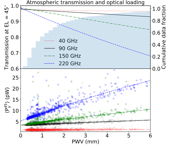
Figure 5. The top plot shows the atmospheric transmission model for each of the CLASS bands (●40 GHz, ●90 GHz, ●150 GHz, and ●220 GHz) as a function of PWV, based on Pardo et al. (2001). The shaded blue histogram indicates the cumulative fraction of CLASS CMB scans acquired below a particular PWV value, with about 80% of data acquired below PWV of 3 mm. The lines plotted on the bottom axes indicate the expected optical loading at 45° elevation for each CLASS band based on: (1) the transmission model shown on the top plot; (2) an atmospheric temperature of 266 K; (3) receiver optical loading offsets of 0.6 pW, 2.4 pW, 2.7 pW, and 4.4 pW at 40 GHz, 90 GHz, 150 GHz, and 220 GHz, respectively; and (4) the brightness temperature to power calibration factors presented in (Dahal et al. 2022). Each data point is the averaged detector optical loading in a CLASS band normalized to 45° elevation. The per-detector optical loading is derived from I - V measurements. The atmospheric transmission model optical loading predictions match well with the I - V optical loading measurements across the CLASS bands.
