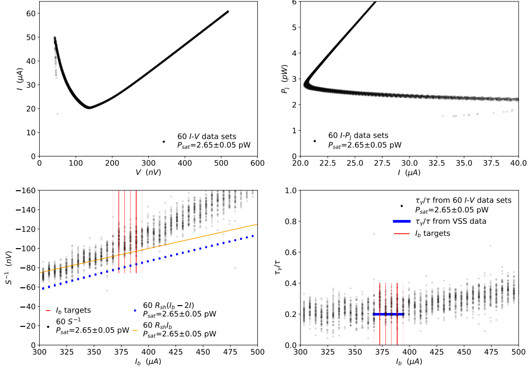
Figure 4. Example of the I - V bin analysis method applied to data from a CLASS Q-band TES. Top left: The black dots plot 60 I - V data sets from the same detector, acquired under almost identical optical loading conditions with the detector saturation power P_{\text{sat}} constrained to 2.65 \pm 0.05 pW. The 60 I - V data sets were acquired between June 2016 and March 2018. Notice that the overlap between the I - V s is almost perfect, except at low TES voltage ( V ) where the detector becomes unstable and moves off its transition to become fully superconducting. The reproducibility of the I - V curves based on their measured P_{\text{sat}} allows us to group them together in bins. We improve the precision of the derived detector parameters by averaging the results across the bin. Having a distribution of equivalent I - V curves simplifies the process of identifying outliers, replacing parameters derived from poor-quality I - V sweeps, and estimating the uncertainty of each derived detector parameter. Top right: The black points show the 60 I - V data sets from the top-left plot, but plotted in terms of bias power P_j on the y-axis and TES current ( I ) on the x-axis. Bottom left: The black points plot the measured I - V responsivity (see Section 2.2.3 and Equation 24) for each I - V in the P_{\text{sat}} = 2.65 \pm 0.05 pW bin shown in the top-left figure. The responsivity is plotted on the y-axis as a function of applied bias current ( I_b ) on the x-axis. The red vertical lines show the target I_b chosen for each of the 60 observation scans following each I - V . As expected, the target I_b chosen for I - V sweeps in the same P_{\text{sat}} bin are similar, validating the algorithm used to set the optimal bias target for each column of detectors. The blue points plot the ideal TES I - V responsivity, while the orange line plots the I_b responsivity. Bottom right: On the y-axis, the black points plot the \tau_\gamma/\tau ratio derived from the I - V s in the P_{\text{sat}} = 2.65 \pm 0.05 pW bin. The ratio is plotted as a function of I_b on the x-axis. The optical time constant \tau_\gamma slows down as the applied I_b increases and the TES equilibrium temperature moves higher on the superconducting transition. Higher on the transition, the electrothermal feedback is weaker, causing the slowdown of the TES response. The blue line plots the measured \tau_\gamma/\tau ratio based on the time constant extracted from the VPM synchronous signal (VSS) (Harrington 2018).
