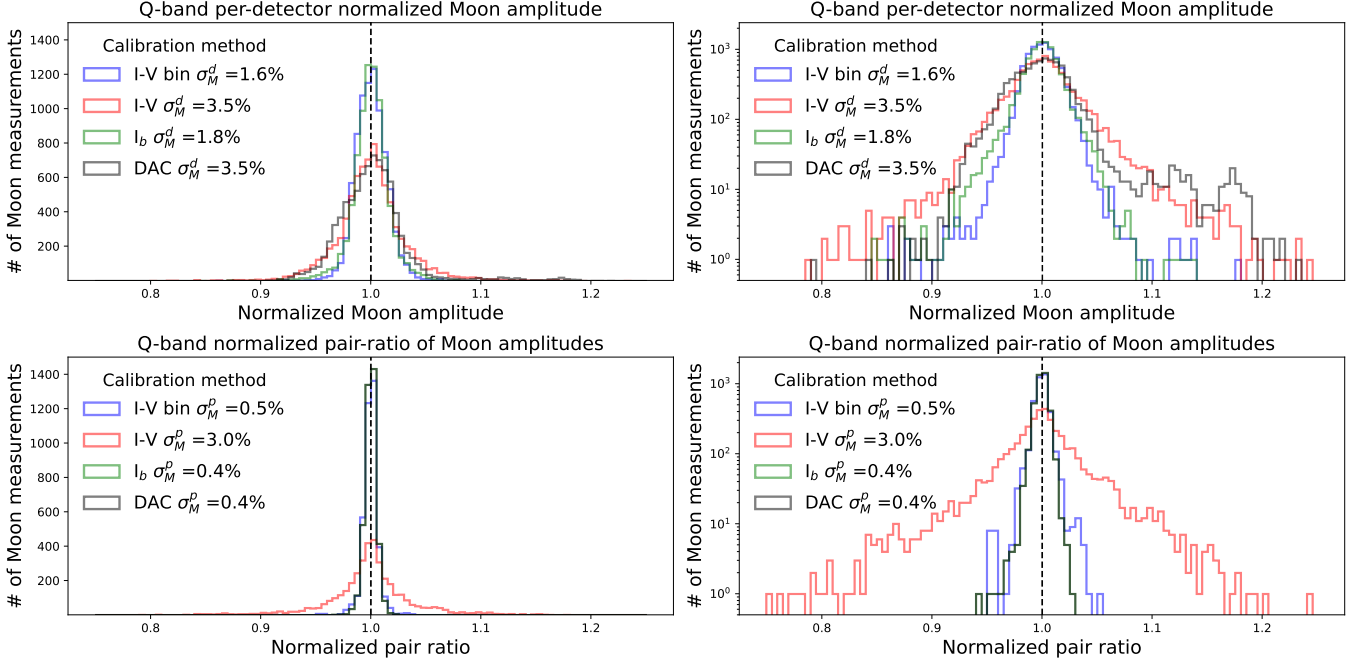
Figure 6. Q-band Moon photometric calibration test histograms. Top row: The x-axis is the per-detector normalized Moon amplitudes across 208 Moon scans acquired between June 2016 and August 2020. The y-axis is the number of Moon measurements in a linear scale on the left and logarithmic scale on the right. Four Moon amplitude histograms are plotted, each corresponding to one of the four calibration models described in the text: I -V bin, I -V, I_b , and DAC. The I_b and I -V bin methods yield the narrowest distribution and thus the most accurate calibrations. These constraints are upper limits on the I_b and I -V bin calibration accuracy, driven by uncertainty in the Moon antenna temperature model. Bottom row: By computing the normalized ratio of Moon amplitudes across detector pairs as shown in the bottom row, the uncertainty of the Moon antenna temperature model is eliminated, and we directly measure the calibration uncertainty between detector pairs. The x-axis is the normalized ratio of Moon amplitudes between detector pairs. The y-axis is the number of Moon ratios on a linear scale on the left and logarithmic scale on the right. The average ratios of each pair are normalized to one. The normalized ratios are then binned across the array, applying the four different calibration methods. The standard deviation values reported in the bottom row legends for ratios of detector pairs are divided by \sqrt{2} for easier comparison to the standard deviations reported on the top row for single detectors.
