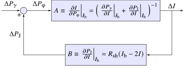
Figure 3. Block diagram of a TES model with negative electrothermal feedback. A < 0 because as I increases ( R decreases), T is suppressed and P_\phi decreases. B > 0 since I_b \gg I due to the voltage bias circuit defined by the shunt resistor R_{sh} \ll R . Therefore AB < 0 , and the feedback is negative. The gain of the feedback loop is A/(1 - AB) = \partial I/\partial P_\gamma|_{I_b} , or 1/S = 1/A - B , which is equivalent to Equation 11. As A approaches negative infinity in the ideal TES case of a perfectly sharp transition, DC responsivity equals -1/B , as expected from Equation 12.
