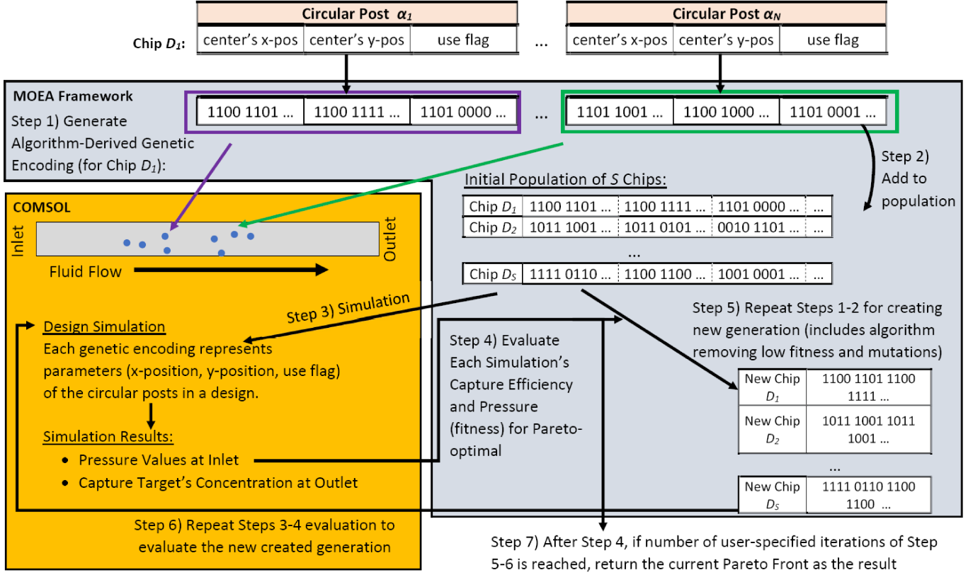
Fig. 5: Overview of our microfluidic capture chip design framework (configured for circular posts). The framework is implemented using NSGA-II, which is integrated into a larger open source Multi-Objective Evolutionary Algorithm (MOEA) framework [22], to enumerate chip designs and maintain a front of Pareto-optimal design points. NSGA-II/MOEA interfaces with finite-element simulation software (COMSOL Multiphysics) which performs the simulation. For each chip, the simulation predicts the concentration of the capture target at each point in the chip (used to quantify how much of the target was captured by the chip) and the pressure that develops at the inlet (which is an indicator of fluid flow resistance as discussed in Figure 2). NSGA-II maintains and evolves a population of encoded chip designs (chromosomes) which encode post positions (genes). Each chip design enumerated by the NSGA-II procedure is simulated by COMSOL Multiphysics, and the results are transmitted back to NSGA-II to update the Pareto Front based on fitness. This process repeats for a user-specified number of generations.
