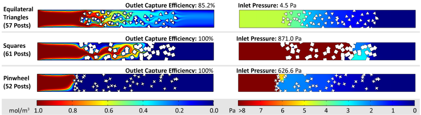
Fig. 15: Simulation results for the highest-capture efficiency chip designs for triangular, square, and pinwheel-shaped posts, discovered during the 4000 design runs reported in Figure 14b. On the left is the predicted concentration of capture target at each location of fluid in the chip during operation. On the right is the predicted pressure at each location of fluid in the chip during operation. Although the triangular posts performed best among the three new shapes in terms of achieve high capture efficiency and low inlet pressure, the highest capture efficiency attained by triangular posts is still lower than the circular post design in Figure 13. Squares and pinwheels are able to obtain maximal capture efficiency, but the inlet pressures are likely to be too large for practical use.
