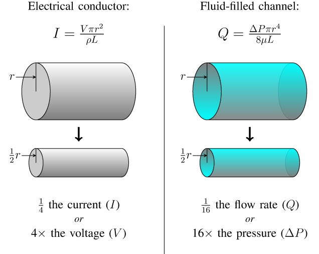
Fig. 2: Comparing the effects of size reduction on electronic and fluidic systems. For an electrical conductor (like a wire, or a trace in an integrated circuit), Ohm’s Law and Pouillet’s Law state that halving the radius r of the conductor causes the conductor to carry \frac{1}{4} the current I (if the voltage applied V is unchanged) or require 4\times the voltage (if the current is to be unchanged). However, for a fluid-filled channel (like those in microfluidic devices), the Hagen-Poiseuille Law dictates that halving the radius of the channel causes the channel to carry \frac{1}{16} the flow Q (if the pressure applied \Delta P is unchanged) or require 16\times the pressure (if the flow rate is to be unchanged). This means that pressure and flow in a microfluidic device are far more sensitive to device design than voltage and current are in an electronic device. Consequently, just as voltage and current are essential aspects of electronic design optimization, pressure and flow must be included in microfluidic design optimization. (The other variables in the equations are constants: L = length of the conductor or channel, \rho = resistivity of the conductor, and \mu = kinematic viscosity of the fluid.)
