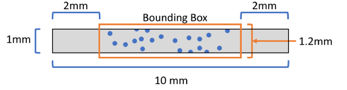
Fig. 4: Chip design constraints used in this study. Fluid flows from left to right through a section of channel that is 1 mm wide and 10 mm long. The bounding box designates the region of the channel where the algorithm can place posts (in this example, 0.2 mm diameter circular posts).
