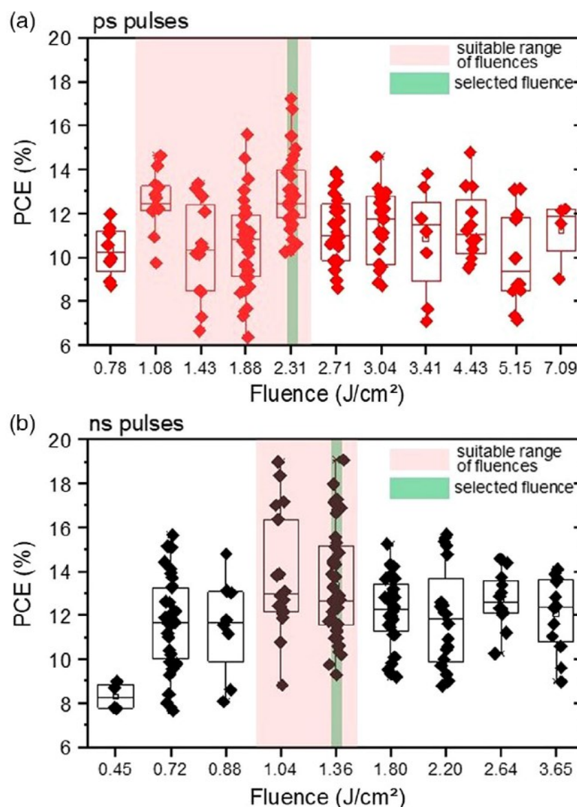
Figure 11. Box-plot of the mini-module PCE as a function of the applied laser fluence for P3 patterning by (a) ps and (b) ns laser pulses [78].
