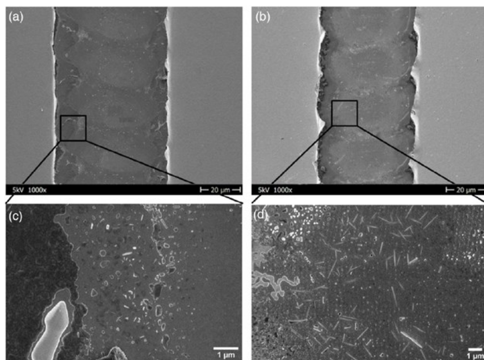
Figure 10. SEM images of the laser-scribed lines patterned by (a) ps and (b) ns laser pulses with fluences of 2.31 and 1.36 J cm -2 , respectively. The black squares schematically show the positions of the high-magnification images of the (c) ps and (d) ns laser scribe lines [78].
