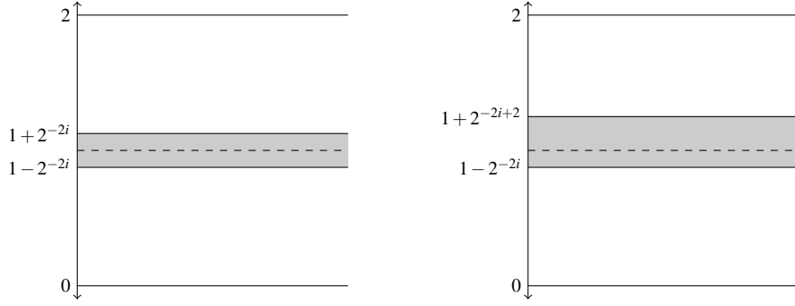
Fig. 2: Schematic representations of the 2 flows where time is shown on the vertical axis. The shaded region corresponds to the times where the vector field is trivial.
