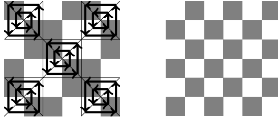
Fig. 1: Action of the flow from t = 0 to t = 1/2 . The shaded region denotes the set \{\rho = 1\}
