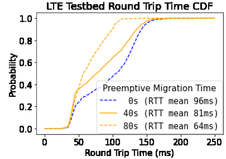
Fig. 16: CDF of user-VM round trip times for different preemptive migration times.
