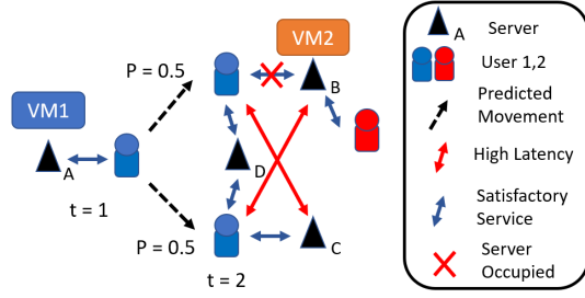
Fig. 2: Challenges of migrations include misplaced migrations due to uncertain mobility, and resource coordination with other users. For example, user 1 may have equal probability of moving close to either servers B or C, while user 2 has occupied resources at server B. Thus, it is optimal to migrate user 1’s VM to server D, to avoid resource conflicts with user 2 and high latencies if the user moves to server B but its VM is migrated to server C.
