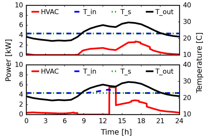
Figure 4. Simulation of HVAC using a grey-box equivalent RC circuit illustrating an uncontrolled operation (top) and a DR event implemented during the summer (bottom) with indoor temperature calculations.
