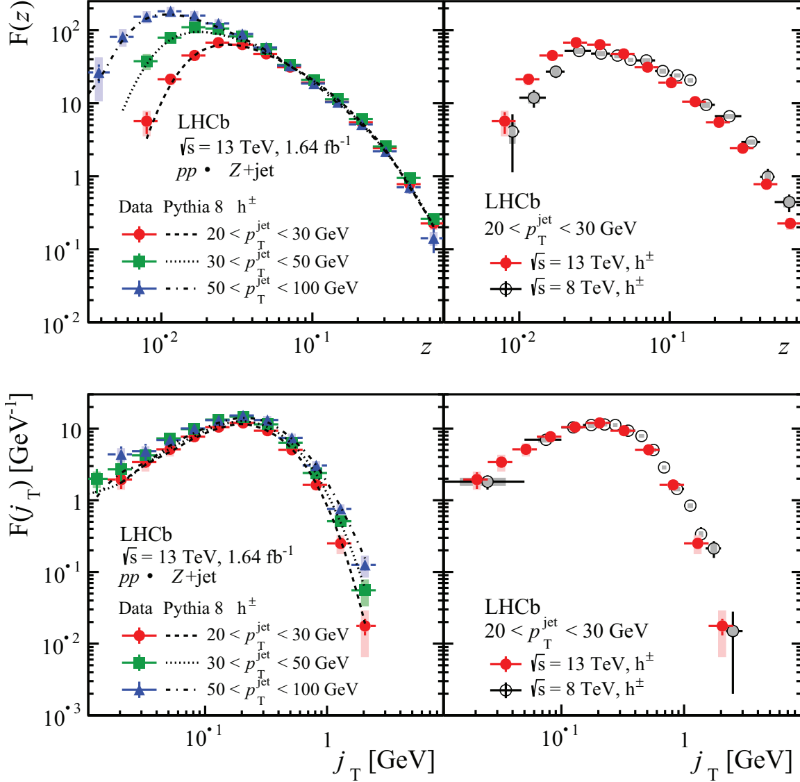
Figure 1: Distributions of (top) the longitudinal momentum fraction and (bottom) the transverse momentum of charged hadrons (pions, kaons, and protons combined) with respect to the jet axis in three jet p_T intervals and (right) comparisons with previous results at \sqrt{s} = 8 TeV for jets with 20 < p_T < 30 GeV [25]. Statistical (systematic) uncertainties are shown in bars (boxes).
